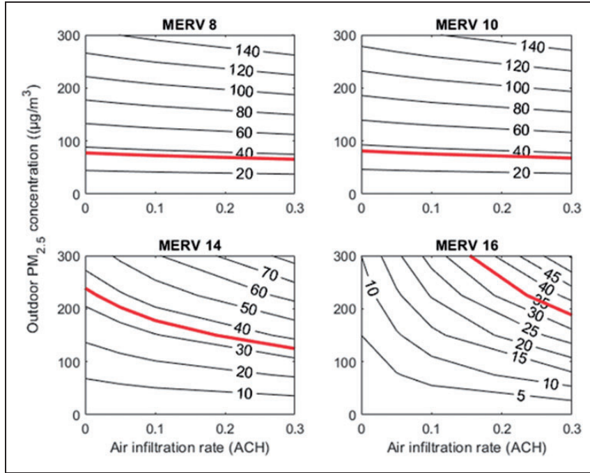
Figure 12. Combined effects of air infiltration rate and filters on the indoor PM_{2.5} concentration under outdoor concentration from 0 to 300 \mu g/m^3 .
