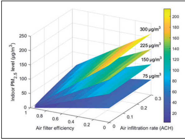
Figure 13. The increasing proportion of indoor PM_{2.5} levels varied with the air infiltration rate and the filter efficiency. (The four surfaces from bottom to top represented the value range of the indoor PM_{2.5} concentration under various air filter efficiency and air infiltration rate when outdoor PM_{2.5} concentration was 75 \mu g/m^3 , 150 \mu g/m^3 , 225 \mu g/m^3 , 300 \mu g/m^3 , respectively.)
