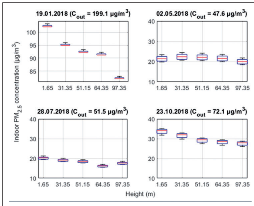
Figure 9. The value range of indoor PM_{2.5} concentration on five selected floors (in order from left to right is 1st, 10th, 16th, 20th, 30 th floor) between 6:00 and 21:00 in four seasons when NPL locates at 50% of the building height (the five horizontal lines for each box in order from top to bottom: maximum value, 3rd quartile, median, 1st quartile, minimum value).
