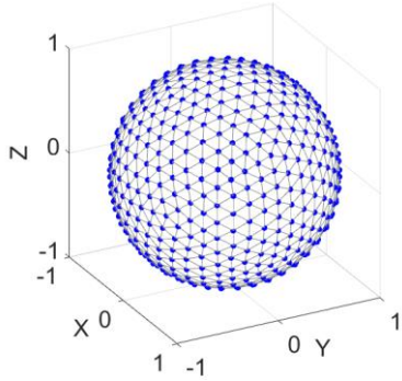
Fig. 4. 642 incident wave directions on a unit sphere are used in the full-wave simulation.
