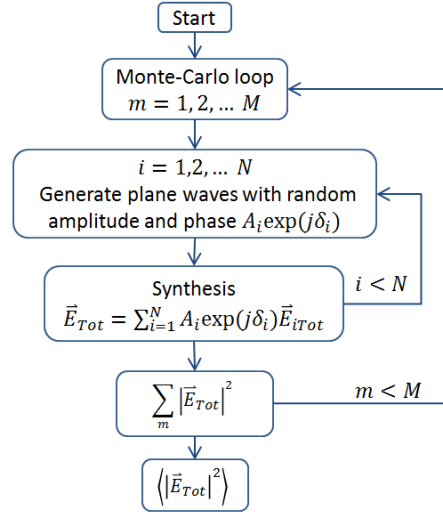
Fig. 3. The workflow of the full-wave Monte-Carlo simulation.
