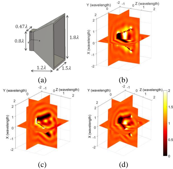
Fig. 12. (a) A horn antenna, (b) simulated \langle |E_{xTot}|^2 \rangle , (c) \langle |E_{yTot}|^2 \rangle and (d) \langle |E_{zTot}|^2 \rangle .
