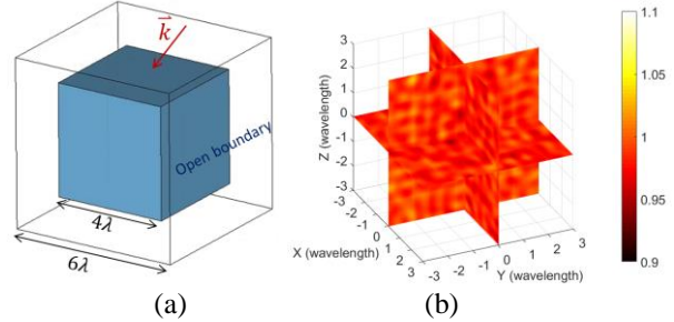
Fig. 5. (a) A vacuum cube, (b) simulated \langle |E_{xTot}|^2 \rangle , the plots for \langle |E_{yTot}|^2 \rangle and \langle |E_{zTot}|^2 \rangle are similar.
