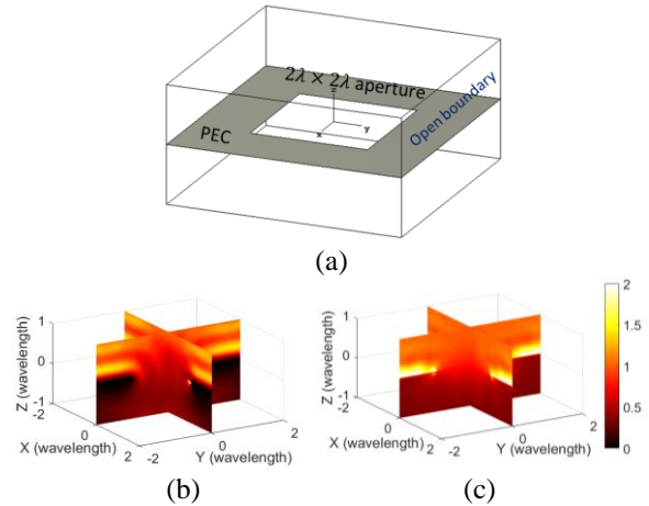
Fig. 13. (a) A half-space aperture, (b) simulated \langle |E_{xTot}|^2 \rangle , (c) simulated \langle |E_{zTot}|^2 \rangle .
