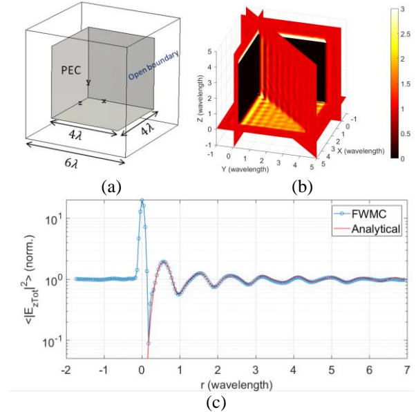
Fig. 8. (a) A right-angle corner, (b) simulated \langle |E_{zTot}|^2 \rangle , (c) a comparison between results from FWMC and analytical equation, note that because of the finite mesh resolution, small error exist when r is close to zero.
