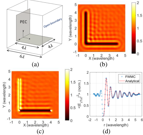
Fig. 7. (a) A right-angle bend, (b) simulated \langle |E_{zTot}|^2 \rangle , (c) simulated \langle |E_{xTot}|^2 \rangle , (d) a comparison between results from FWMC and analytical equation.
