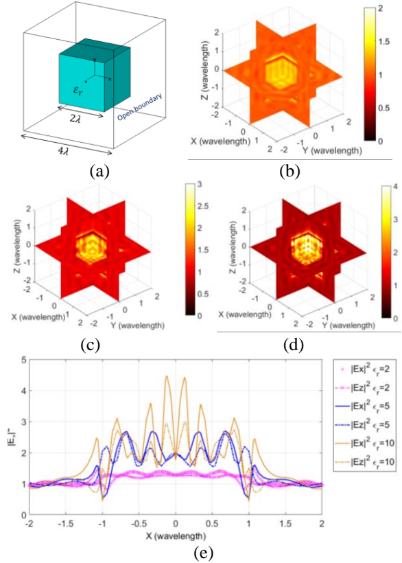
Fig. 10. (a) A dielectric block with relative permittivity \epsilon_r , simulated \langle |E_{zTot}|^2 \rangle for (b) \epsilon_r = 2 , (c) \epsilon_r = 5 and (d) \epsilon_r = 10 , (e) extracted plots on the line y = 0, z = 0 , \langle |E_{yTot}|^2 \rangle are not shown as they are the same as \langle |E_{zTot}|^2 \rangle .
