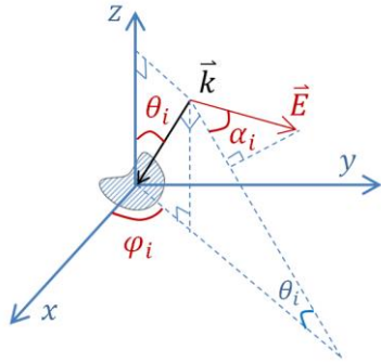
Fig. 2. Angle definitions of an incident plane wave.
