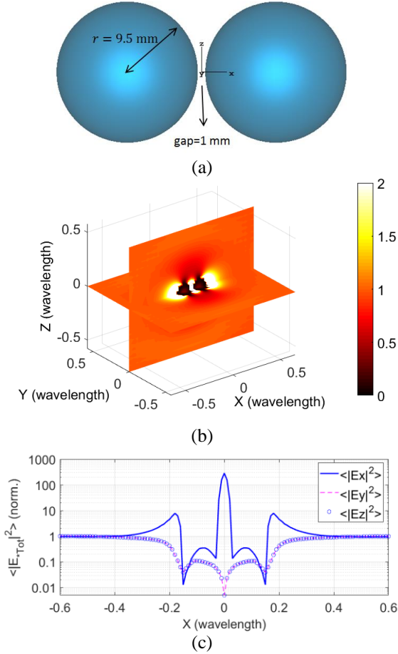
Fig. 11. (a) Two spheres gapped with 1 mm, the material is set as sea water, (b) simulated \langle |E_{xTot}|^2 \rangle , (c) extracted plots on the line y = 0, z = 0 .
