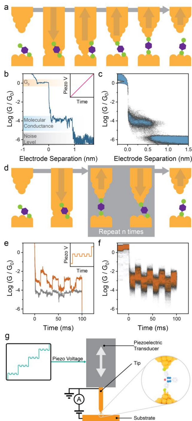
Figure 2: Experimental methods. (a) Schematic depiction of a linear-ramp break-junction measurement. The two electrodes are brought together and then pulled apart in the presence of molecules with appropriate contacts, resulting in the formation of molecular junctions. (b) Example conductance trace during a break-junction experiment (piezo signal in inset), where the G_0 plateau is followed by a molecular plateau several orders of magnitude less conductive. Thousands of these traces are acquired and compiled in (c) conductance vs. electrode separation density plots. (d) Schematic depiction of a piezo-modulation break-junction measurement. As the junction is fabricated, the relative position of the electrodes is modulated n times before rupture. (e) Example conductance vs time trace of a piezo-modulation measurement. A mechanoresistive molecule (orange) shows conductance variations in phase with the piezo signal (inset), while modulating a non-mechanoresistive molecule (grey) only results in increased noise. Thousands of these traces are collected and compiled in conductance vs. time density plots (f). (g) Experimental setup for piezo-modulation experiments in a STMBJ configuration, where a custom ramp is applied by an arbitrary waveform generator to the piezoelectric transducer responsible for moving the STM tip.
