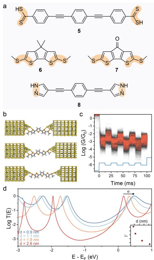
Figure 4: Switch between denticity at multifunctional electrode contacts. (a) Structures of the bifunctional molecular wire termini discussed in this review. The bidentate system is highlighted in orange. (b) Evolution of a junction fabricated with (methylthio)thienyl contacts as the electrodes are driven apart. The molecule-electrode interface evolves from a bidentate-bidentate configuration to bidentate-monodentate and finally monodentate-monodentate before junction rupture. (c) Example conductance vs time density map for compound 7 , with the 0.3 nm modulation piezo signal superimposed in light blue. Conductance is modulated in phase by approximately one order of magnitude, as the molecule is cycled between different configurations. (e) Transmission curves for the \alpha -terthienyl derivative shown in (b), where the effect of the junction size on the parameters \sigma and \Gamma of Eq. 2 can be appreciated. The evolution of \Gamma as a function of junction stretching is shown in the inset. Panels (b)-(e) replotted from data publicly available in Ferri et al. 65
