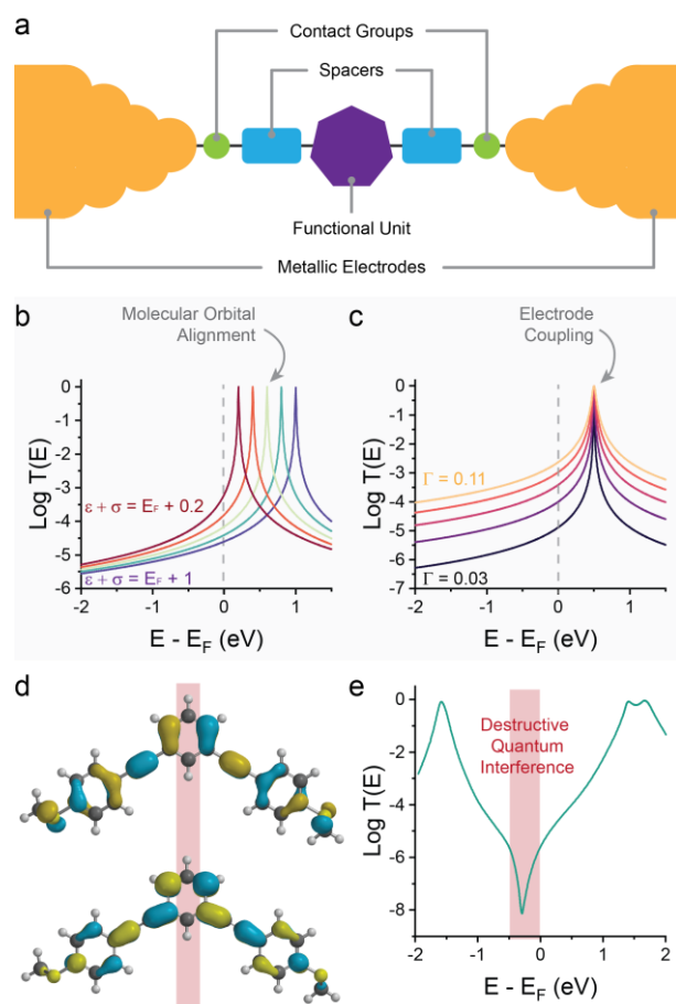
Figure 1: Fundamental concept of charge transport in molecular wires. (a) Anatomy of a molecular junction, showing the electrodes “chemically soldered” to a functional unit by the use of contact groups (with or without the use of spacers). (b) example of T(E) as the orbital energy is moved closer to the Fermi level of the electrodes. (c) example of T(E) as the coupling parameter \Gamma is increased. (d) Molecular orbitals (HOMO = top; LUMO = bottom) for a meta -connected molecular wire (1,3-bis((4-(methylthio)phenyl)ethynyl)benzene) and (e) resulting DFT-calculated T(E) for its Au-molecule-Au junction. Panels (b) and (c) calculated with equation 2. Molecular orbitals in (d) calculated with Wavefunction Inc. Spartan 18, DFT \omega B97X-d/6-31G*. Data in panel (e) digitised from Jiang et al. 22 and replotted.
