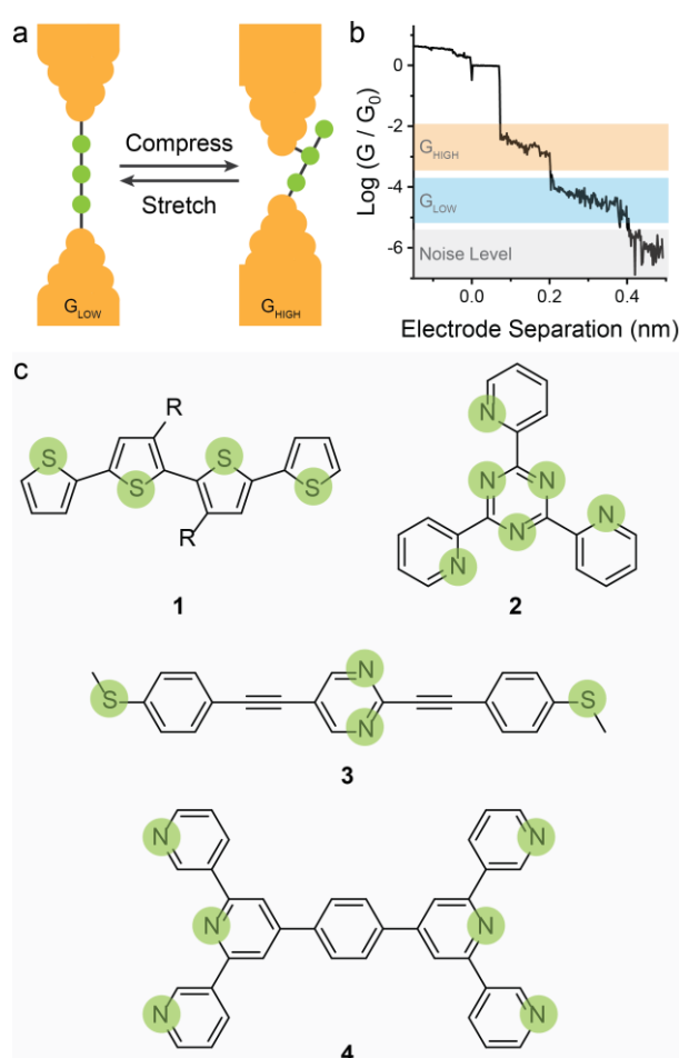
Figure 3: Switch between contact groups spaced along the conductive backbone. (a) depiction of a junction with three possible contact groups and its structure in a relaxed and compressed junction conformation. (b) Example STMBJ trace for the compounds depicted in (a), where after rupture of the atomic contact, the molecule adopts the compressed conformation, and it relaxes to an extended structure as the electrodes are driven apart. Further increase of the electrode separation results in junction rupture and decay of the conductance to the noise level of the instrument used. (c) Structures of molecules with mechanoresistive functionality based on sequential switching between different contact groups. The possible contact points are highlighted in green.
