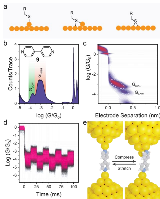
Figure 5: Switch between different contact configurations at the molecule-electrode interface. (a) possible thiol binding mode on Au surfaces. (b) Conductance histogram for 4,4'-dipyridyl (structure shown as inset) and (c) its 2D conductance vs electrode separation density map. A bimodal
