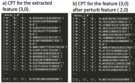
Figure 4: A toy example, with only three intervals for each feature, illustrates the conditional probability table for the first extracted feature from layer dense_1 before and after shifting intervals of feature (2, 0) in the dataset used to fit the BN.
