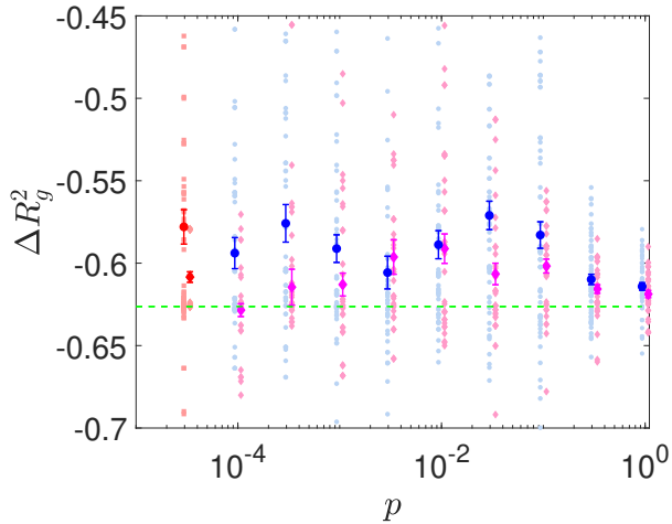
FIG. 3: Distribution (mean and standard error) of relative shrinkage \langle \Delta Rg^2 \rangle against the rewiring probability p of the generated Watts-Strogatz networks. 50 trials were tested for each rewiring probability by generating a new network of N = 1000 (shown in blue or circle markers
