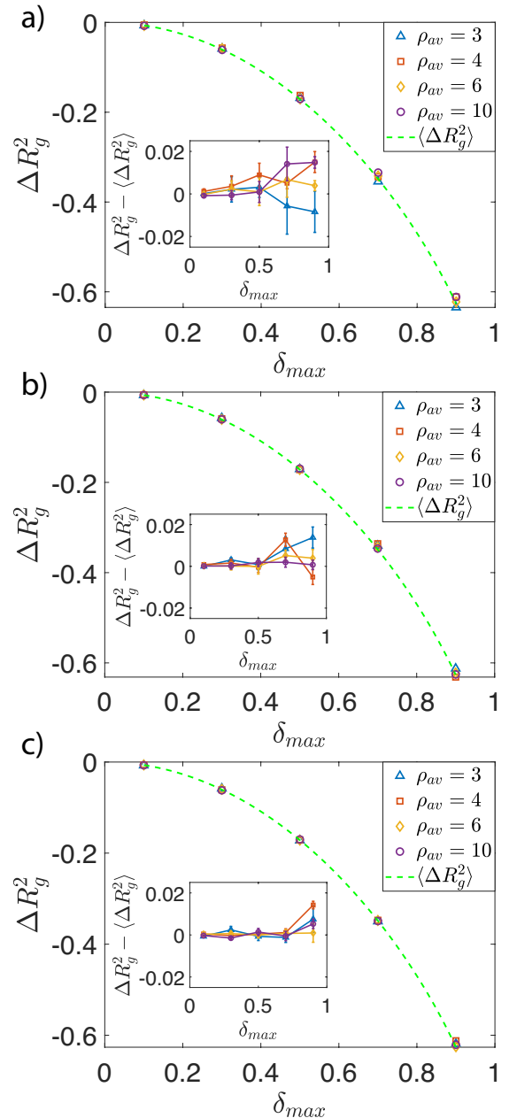
FIG. 2: a) Variation of the relative shrinkage \Delta Rg^2 < 0 against the maximum prestrain \delta_{max} for networks of N = 500 masses while b) and c) show similar results of tests done for N = 2000 and N = 4000 respectively. The dotted green line represents the expectation calculated using Eq. (12) and the solid lines refer to numerical simulations. Networks of different average coordination numbers, \rho_{av} are shown by the different markers. Each marker shows the mean of 6 trials with separate realisations of networks, generated according to the Watts-Strogatz (rewiring probability p = 0.7 ). The error bars represent the Standard Error. The inset shows the difference between the expected relative shrinkage and the shrinkage from the numerical simulations \Delta Rg^2 - \langle \Delta Rg^2 \rangle .
