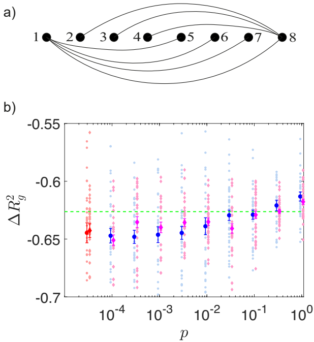
FIG. 5: a) Sketch of of an End-Hub network of size N = 8 with H = 1 hub on either side. b) Distribution (mean and standard error) of relative shrinkage \langle \Delta R_g^2 \rangle against the rewiring probability of the generated End-Hub networks with H = 3 hubs per side of the network. 35 trials were tested for each rewiring probability by generating a new network of N = 1000 nodes (shown in blue or circle markers
