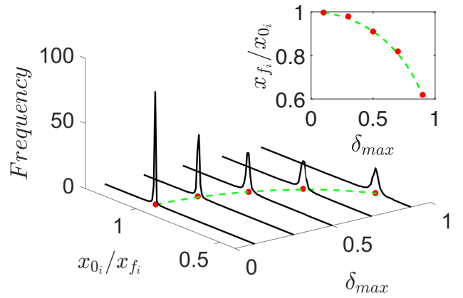
FIG. 1: Comparison between theoretical predictions and numerical results. The solid black lines show histograms of x_{f_i}/x_{0_i} plotted for all nodes of the network. For each of the values of maximum noise \delta_{max} shown, a new network was generated and tested according to the method outlined in the text. Each of the tested networks has N = 2000 masses and have been created according to the Watts-Strogatz strategy [24] with rewiring probability p = 0.7 . The dotted green line represents the expected shift per node, 1/\psi , against \delta_{max} . The circle markers show the mean of each of the histograms. A top view of the plot is shown in the inset.
