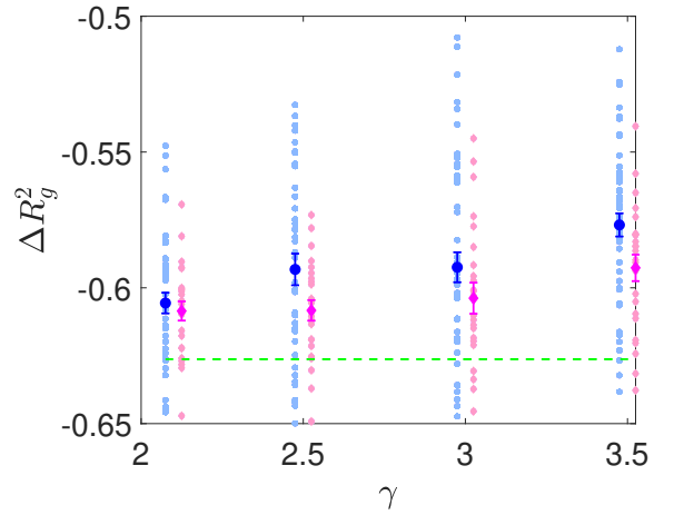
FIG. 4: Distribution (mean and standard error) of relative shrinkage \langle \Delta Rg^2 \rangle against the degree exponent \gamma of the generated scale-free networks. 50 trials were tested for each \gamma by generating a new realisation of a network of N = 2000 for each trial. The prestrain strength was set to the maximum \delta_{max} = 0.9 and dotted green line is the expectation given by the theory. N = 2000 is shown in magenta (or diamond markers)
