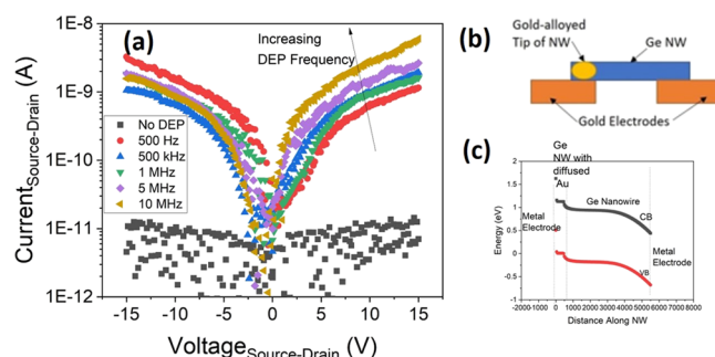
Figure 2. (a) IV characteristics of as-fabricated Ge nanowire FETs at differing DEP frequencies with an ungrounded gate potential, (b) representation of contacted NWs, and (c) schematic of the resulting band alignment.
