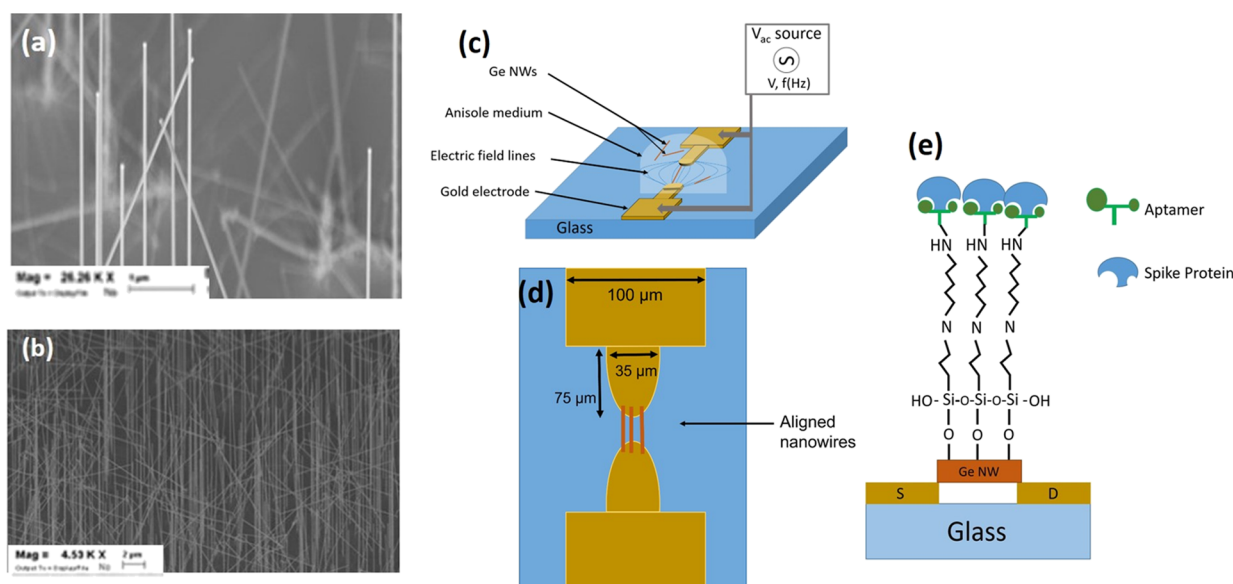
Figure 1. (a) and (b) SEM images of typical as-grown Ge NWs, (c) overview schematic of DEP system (not to scale), (d) top view schematic of final device (not to scale), and (e) side profile of the final device with functionalization (not to scale).
