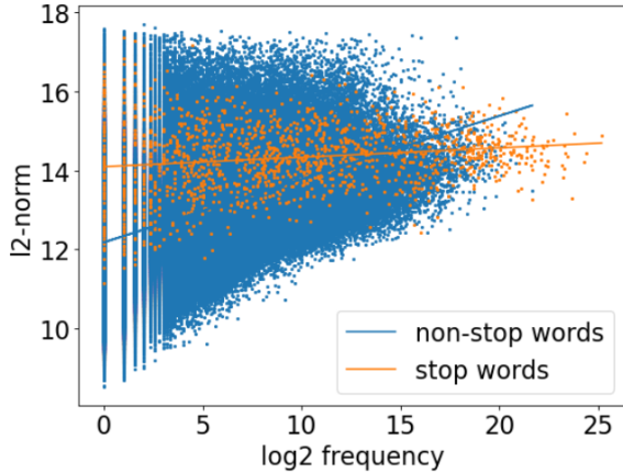
Figure 2: \ell_2 norm of the averaged contextualised word embedding of a word against its log-frequency in the pretrain corpus. Stop words and non-stop words are shown respectively in orange and blue dots. Lines of best fits for each category are superimposed.
