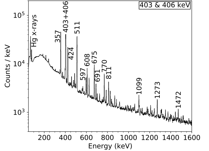
FIG. 19: Portion of the \gamma -ray energy spectrum gated on the 403-keV ( 4_1^+ \rightarrow 2_1^+ ) and 406-keV ( 2_1^+ \rightarrow 0_1^+ ) \gamma -ray transitions in ^{186}\text{Hg} . The most prominent lines have been labeled with the transition energy in keV.
