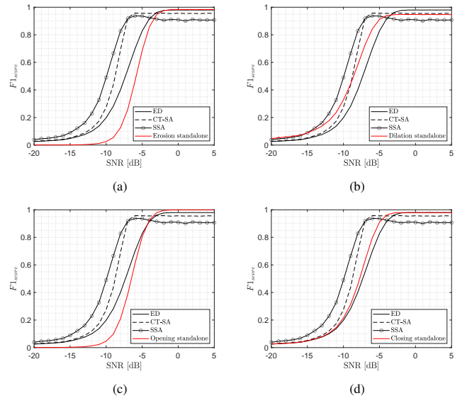
Figure 12: MOs as standalone SAE methods: (a) erosion, (b) dilation, (c) opening, and (d) closing.
