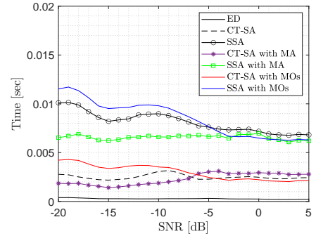
Figure 16: Computation time of the proposed MO-based SAE method.
