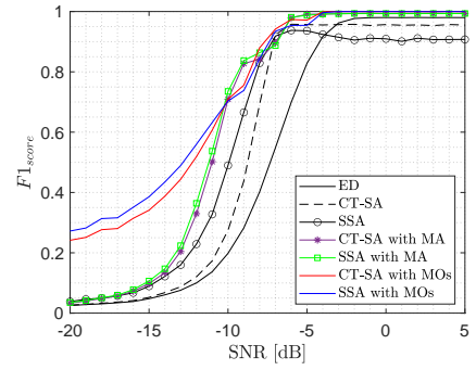
Figure 15: F1 score of the proposed MO-based SAE method.
