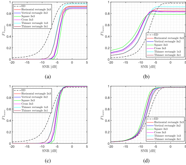
Figure 6: F1 scores with different shapes of SE for MOs as standalone SAE: (a) erosion, (b) dilation, (c) opening, (d) closing.
