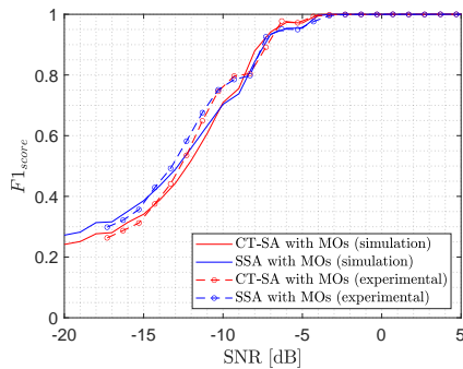
Figure 17: Experimental validation of the proposed method.
