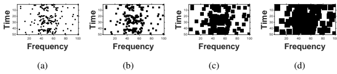
Figure 10: Dilation at SNR = -10 dB using a squared SE for the SAs shown in Fig. 3a: (a) extra small, (b) small, (c) medium and (d) large.
