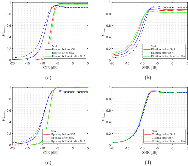
Figure 14: MOs as pre/post-processing to SSA: (a) erosion, (b) dilatation, (c) opening, and (d) closing.
