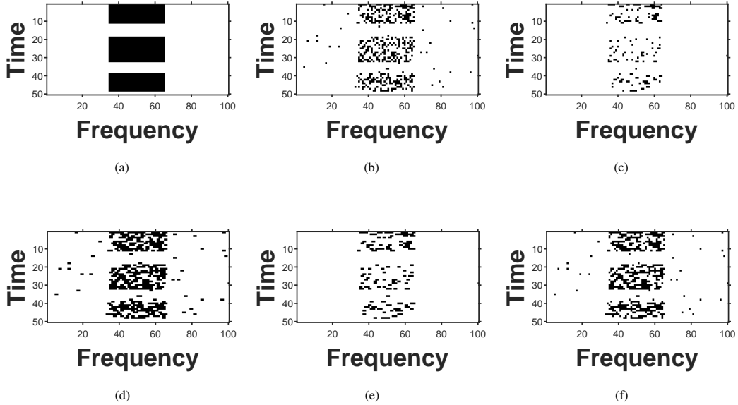
Figure 3: Several versions of the same time/frequency grid: (a) Original generated by transmitter, (b) Observed at receiver after ED (with threshold set for P_{fa} = 1\% ) at SNR = -7 dB ( P_d \approx 0.39 ), (c) Eroded at the receiver with a 1 \times 2 rectangular SE, (d) Dilated at the receiver with a 1 \times 2 rectangular SE, (e) Opened at the receiver with a 1 \times 2 rectangular SE, (f) Closed at the receiver with a 1 \times 2 rectangular SE.
