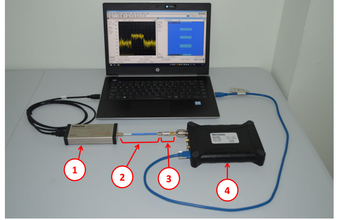
Figure 5: Experimental platform used in this work: (1) vector signal generator, (2) coaxial cable, (3) attenuator, and (4) spectrum analyzer.
