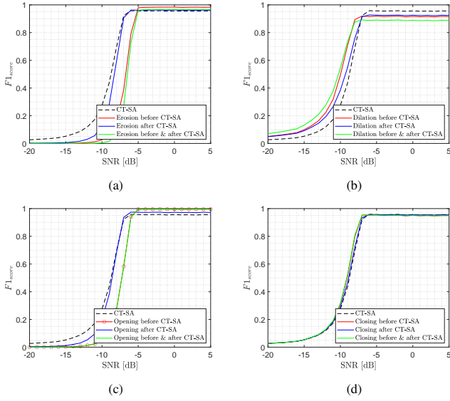
Figure 13: MOs as pre/post-processing to CT-SA: (a) erosion, (b) dilatation, (c) opening, and (d) closing.
