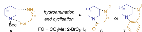
Figure 1: Bicyclic twisted amides and anilines, and a proposed modular approach to congeners.
