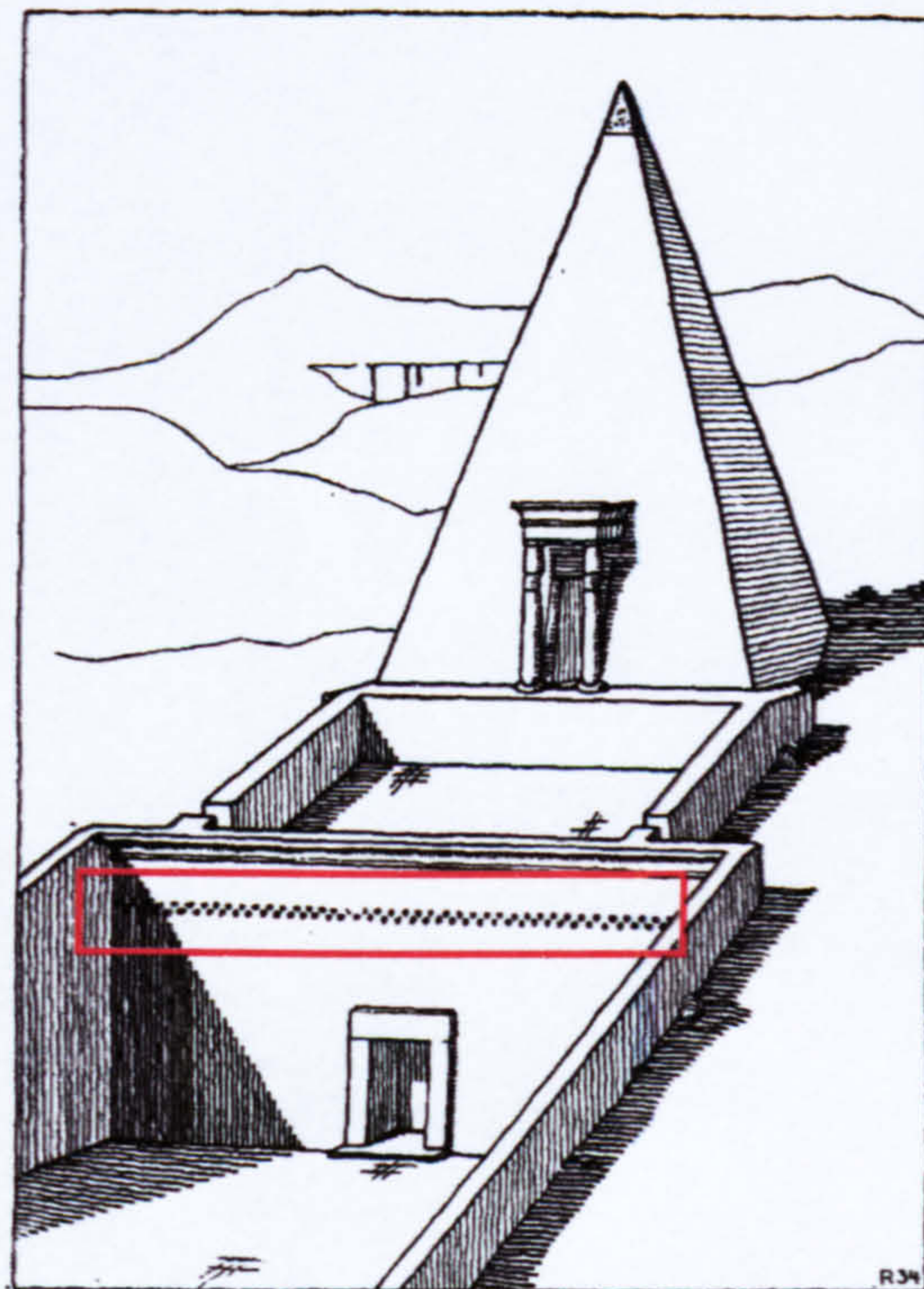
Figure 9 – Reconstruction of TT288/9 (after Borchardt et al, 1934, 29 Abb.6)
