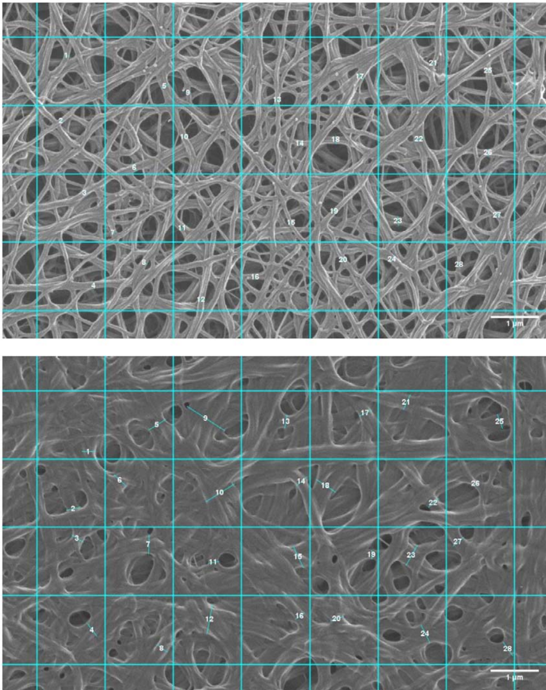
Figure 2: Fibrin fiber diameter measurement scheme. SEM micrographs of a prepared PPP clot from a representative healthy control (top) and RA (bottom).
