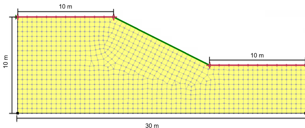
Fig. 5. Finite element model for slope in example 1
