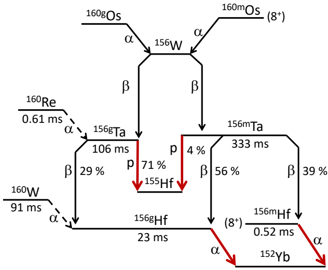
Figure 1: Schematic diagram showing the expected \alpha -decay chain of ^{160}\text{Os} . The labels g and m in the superscripts denote ground and isomeric states, respectively. The \alpha decays of both the ground state and the isomeric state of ^{160}\text{Os} are expected to populate the ground state of the unknown nuclide ^{156}\text{W} , which is predicted to \beta decay [12]. The red arrows denote the decays that were considered in the search for the \alpha decay of ^{160}\text{Os} , namely the proton-decay branches of ^{156g,156m}\text{Ta} and the \alpha decays of ^{156g,156m}\text{Hf} . The dashed arrows indicate the \alpha decays of ^{160}\text{Re} and ^{160}\text{W} , which would be expected in correlated energy spectra together with ^{160}\text{Os} \alpha decays. The half-life for the isomeric state in ^{156}\text{Ta} is from the present work. Other half-lives and branching ratios are taken from Refs. [5, 36].
