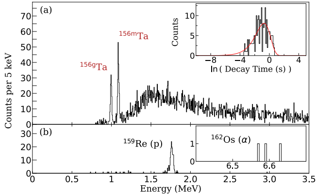
Figure 3: Energy spectra of decays measured in the DSSD. Peaks are labelled with their assignments. (a) Decays that were followed by an \alpha decay of ^{155}\text{Lu} in the same pixel in the measurements with the ^{102}\text{Pd} target. See text for details of the timing conditions. The broad distribution extending to higher energies is from the decays of ^{159}\text{W} nuclei in which the \alpha particles escape from the DSSD without depositing their full energy. The inset shows the distribution of the time differences between ions being implanted and events in the ^{156m}\text{Ta} proton-decay peak in the same DSSD pixel. The red curve shows the fit to this time distribution. (b) Decays occurring within 370\ \mu\text{s} of an ion being implanted into the same DSSD pixel that were followed within a further 12.5 ms by an \alpha decay of ^{158}\text{W} in the measurement with the ^{106}\text{Cd} target. The only clear peak below 3.5 MeV is from proton decays of ^{159}\text{Re} . The inset shows a higher-energy region of the spectrum, in which a few \alpha decays of ^{162}\text{Os} can be seen.
