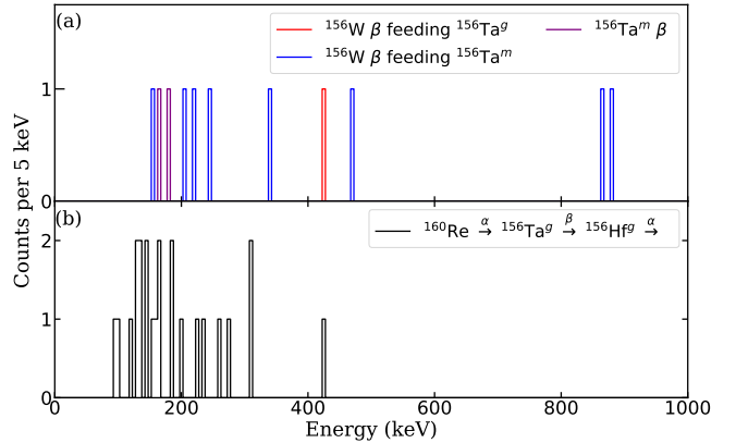
Figure 4: (Colour online) (a) Energy spectrum of the \beta -decay events presented in Table 1. The colours indicate the assignments to specific \beta -decaying states. (b) Energy spectrum of \beta particles observed within 530 ms of an \alpha decay of ^{160}\text{Re} and followed within 115 ms by an \alpha decay of the ground state of ^{156}\text{Hf} .
