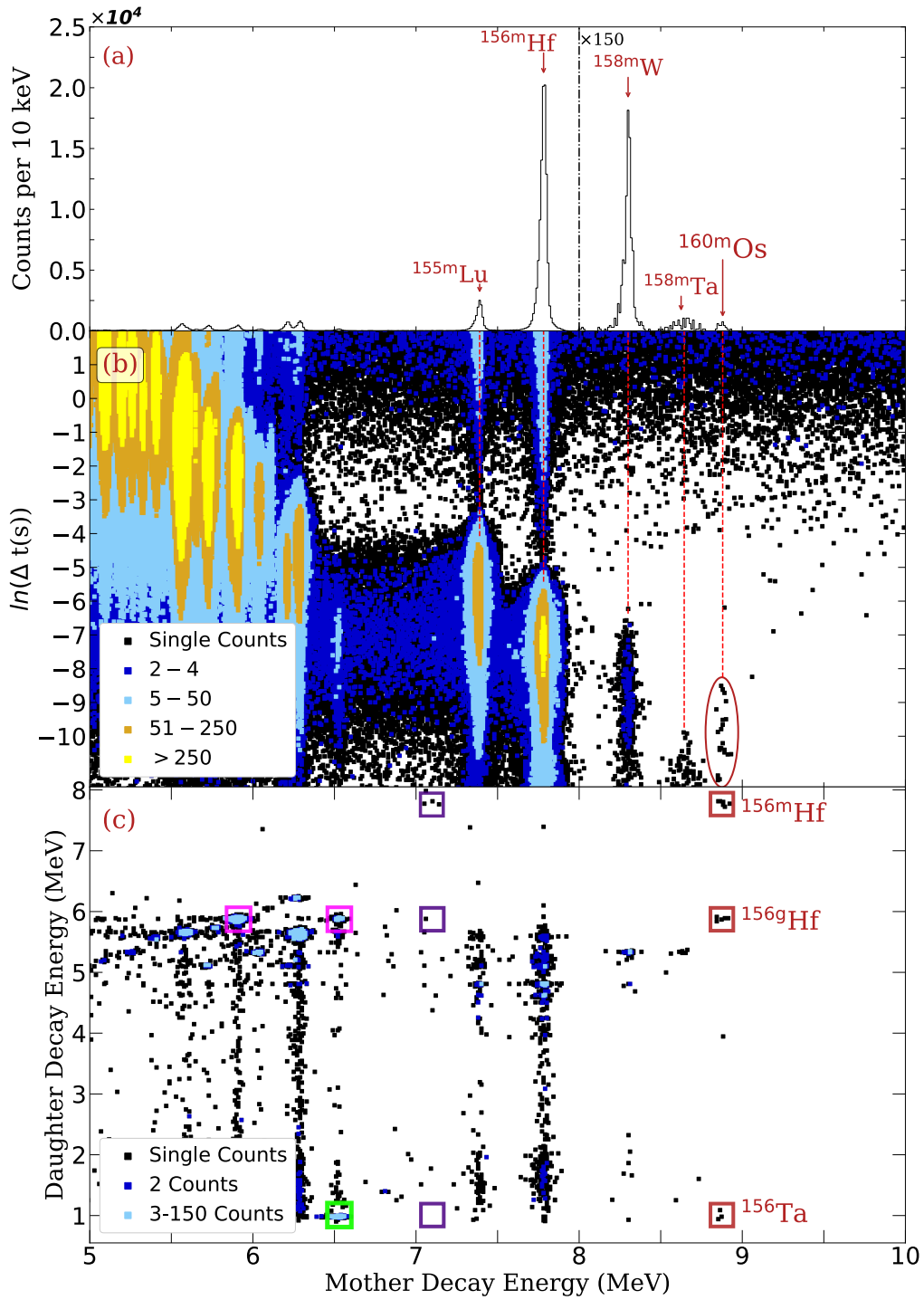
Figure 2: (a) Energy spectrum of \alpha decays measured in the DSSD within 250 \mu\text{s} of an ion being implanted into the same pixel. Peaks are labelled with their assignments. Note the expanded vertical scale to the right of the dot-dash line. (b) The energies of \alpha decays plotted against the natural logarithm of the time difference between the \alpha decay and the preceding evaporation residue implanted into the same DSSD pixel. The dashed lines are drawn to guide the eye to the \alpha decays of the spin-gap isomers of ^{155}\text{Lu} , ^{156m}\text{Hf} , ^{158m}\text{W} , ^{158m}\text{Ta} and the events in the ellipse that are assigned as \alpha decays of the isomer in ^{160}\text{Os} . (c) Correlation matrix of “mother” \alpha -decay events occurring within 400 \mu\text{s} of an evaporation residue being implanted into the same DSSD pixel with “daughter” decays occurring within a further 1.75 s in the same pixel. Note that the minimum energy threshold was set in software to exclude \beta -decay events from these correlations. The candidate ^{160}\text{Os} \alpha decays can be seen to fall within the 3 groups inside the red squares corresponding to daughter proton decays of ^{156}\text{Ta} and the \alpha decays of the ground state and isomeric state of ^{156}\text{Hf} . The corresponding correlations of the \alpha decays of the ground state of ^{160}\text{Os} are indicated by the purple squares. The green square highlights \alpha decays of ^{160}\text{Re} correlated with proton decays of the ground state of ^{156}\text{Ta} , while the magenta squares highlight \alpha decays of ^{156}\text{Hf} that are preceded by the \alpha decays of ^{160}\text{Re} and ^{160}\text{W} . Note that the energy scales are valid for \alpha decays and therefore give apparent proton energies that are \sim 40 keV too low.
