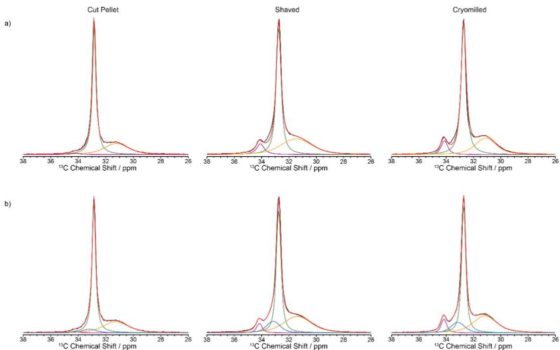
Figure 2. ^{13}\text{C} CP MAS spectra of virgin HDPE cut pellet, shaved and cryomilled samples at 9.4 T with a 2 ms contact time. Experimental spectrum (black), totally fit (red) with a) 3 components and b) 4 components are shown (orthorhombic in green, amorphous phase in orange, monoclinic in purple and interphase in blue).
