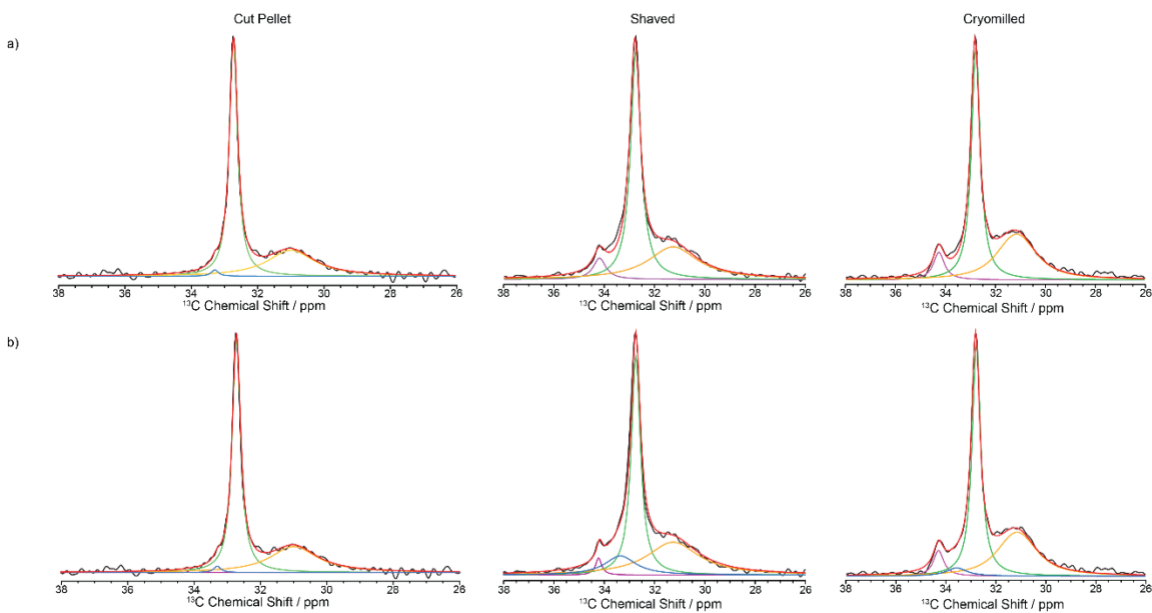
Figure 7. ^{13}\text{C} directly excited spectra of virgin HDPE cut pellet, shaved and cryomilled samples at 9.4 T. Experimental spectrum (black), totally fit (red) with a) 3 components and b) 4 components are shown (orthorhombic in green, amorphous phase in orange, monoclinic in purple and interphase in blue).
