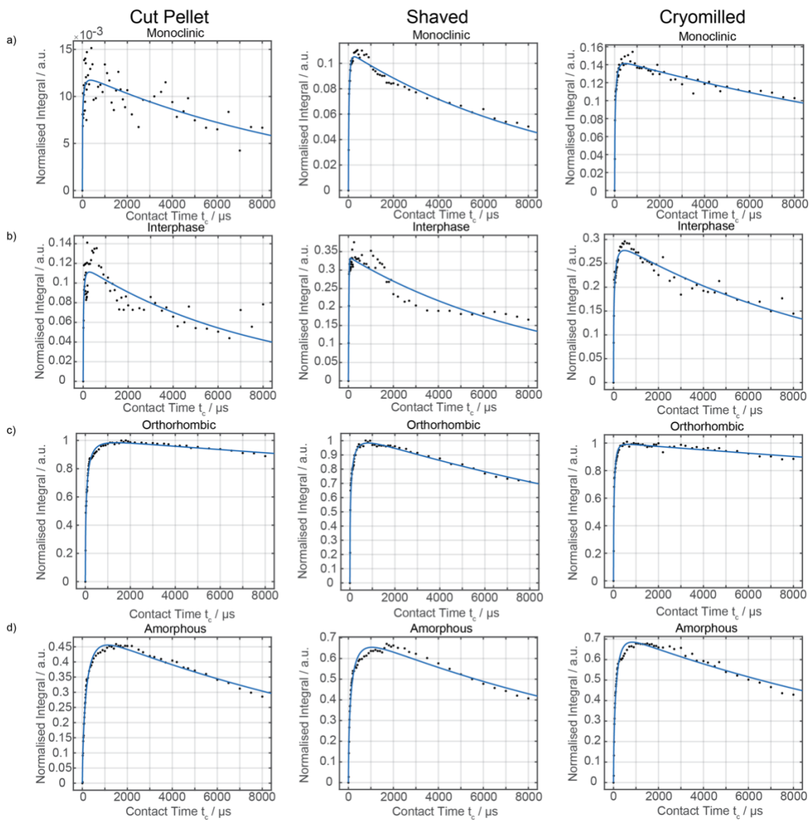
Figure 6. ^{13}\text{C} CP build-up curves for the virgin HDPE cut pellet, shaved and cryomilled samples at 9.4 T for all four domains of the a) monoclinic, b) Interphase c) orthorhombic and d) amorphous regions. Experimental data points are given in black circles fitted to the simplest CP kinetics model (blue curve) as described in the Materials and Methods section and are normalised against the most intense signals of the orthorhombic domain.
