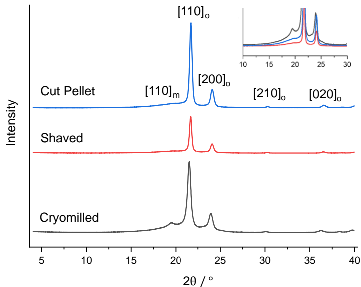
Figure 4. Powder XRD patterns for the cut pellet, shaved and cryomilled samples. The Miller indices of the reflections are given in square brackets where the subscripts m and o correspond to the monoclinic and orthorhombic phases. The insert shows a magnified view of the amorphous domain in the powder XRD patterns.
