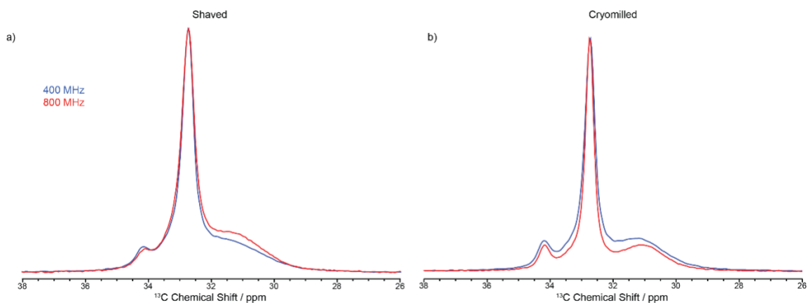
Figure 3. Spectral comparison between CP experiments conducted 9.4 T (blue) and 18.8 T (red) for the a) shaved samples and b) cryomilled samples, all collected using a contact time of 2 ms.
