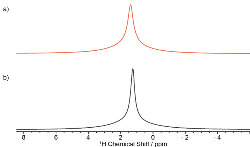
Figure 5. ^1\text{H} MAS Hahn-echo spectra of a) shaved (red) and b) cryomilled (black) samples obtained at 18.8 T. The ^1\text{H} MAS NMR spectrum of the cut pellet was not recorded due to the larger size of the pellet than the 1.3 mm rotor used.
