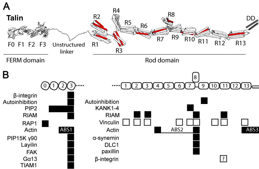
Figure 1. Talin domain organization and interactions. (A) Talin contains an N-terminal FERM domain (F0–F3) connected via an 80-aa unstructured linker to the 13 talin rod domains R1–R13. 9 of the 13 rod domains contain VBSs (red). (B) Major binding sites for folded talin domains (black boxes) and unfolded domains (white boxes).
