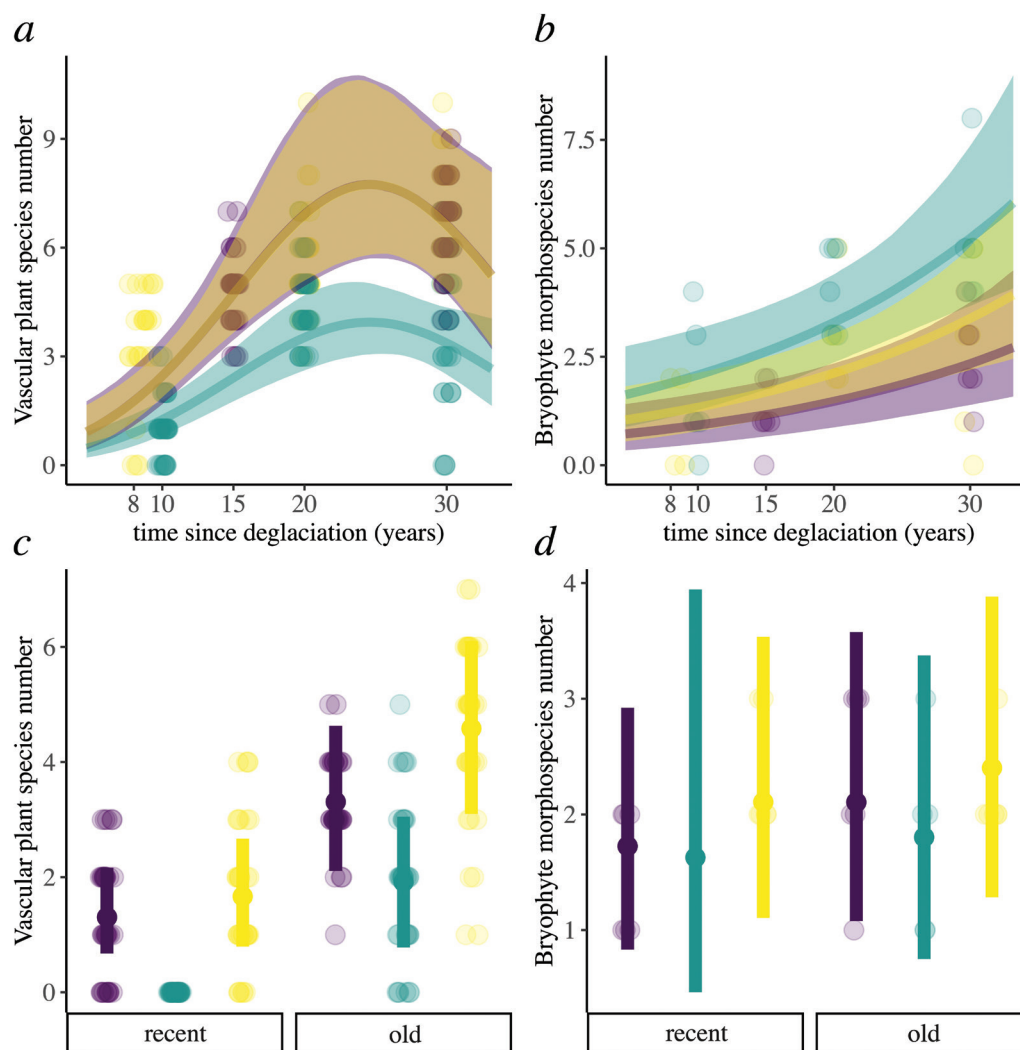
Figure 4. Effect of time since deglaciation ( tsd in years) on the number of vascular plant species and bryophyte morpho-species at tidewater ( a, b ) and inland ( c, d ) glacier sites modelled with Bayesian Inference. Transparent points represent the original data. Lines ( a, b ) or points ( c, d ) are the estimated mean effects of tsd . Purple, turquoise and yellow areas ( a, b , Harker: purple, Lyell: turquoise, Nordenskjöld: yellow) or intervals ( c, d , Husvik: purple, Col: turquoise, Hodges: yellow) represent the Bayesian 95% credible intervals, respectively.
