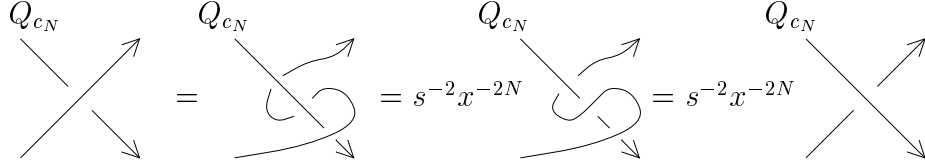
Figure 5.3: Pulling a differently oriented arc through a component decorated with Q_{c_N} .
