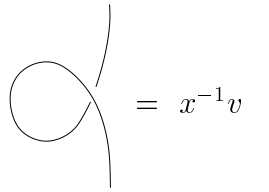
Figure 2.7: A derived relation in \mathcal{S}(\mathcal{F}, \Gamma) .
