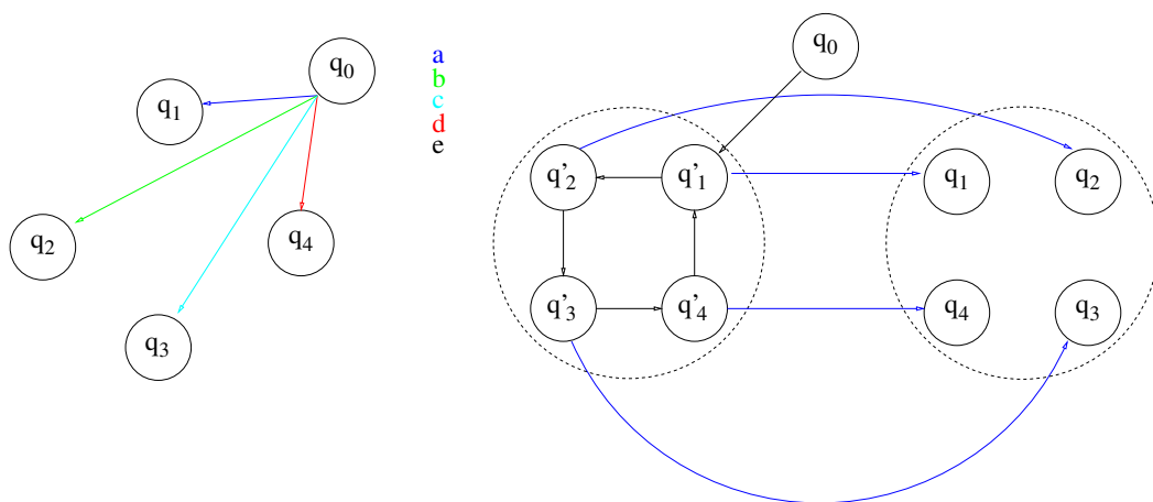
FIGURE 2.3: The above diagram depicts an equivalent, multi-alphabet, asynchronous automaton and a single alphabet, with epsilon transitions, synchronous automaton. Symbols, a , b , c , d and e , the epsilon transition, are colour coded such that receipt of the symbol a is signified by a blue edge.
