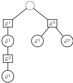
Figure 2: Factored Statistics: joint histories are maintained (for specific joint actions and observations specified by \vec{a}^j and \vec{\sigma}^k ), but action statistics are factored at each node.
