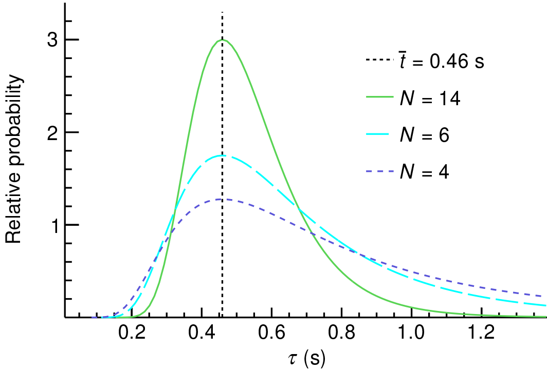
Figure A.4: (Color online) Likelihood functions for \tau if different number of decay chains N are measured to have an average lifetime \bar{t} = \bar{t}_1 = 0.459 s. The (green) solid line corresponds to the \tau likelihood function for decay step j = 1 in the data set of fourteen short chains. The functions are normalised such that the integral on the interval [0, \text{inf}] is one.
