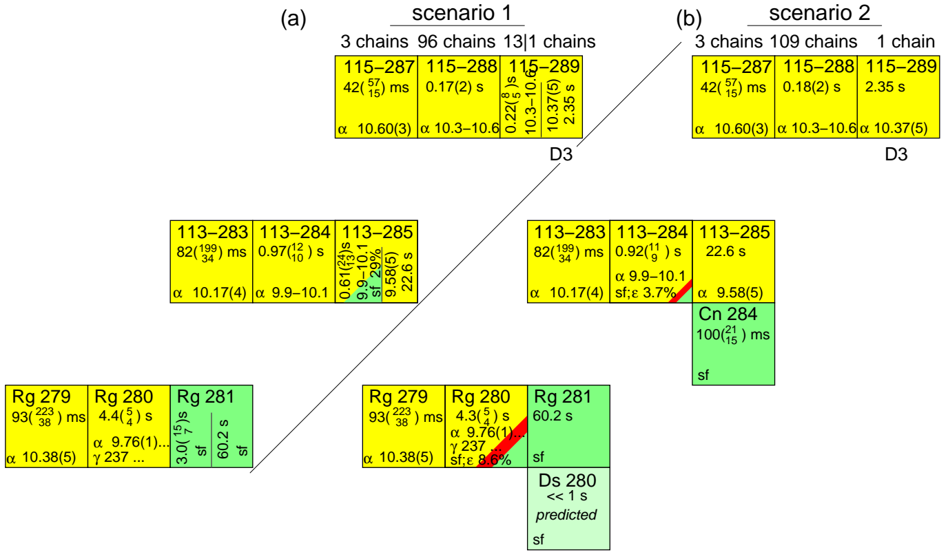
Figure 2: (Color online) Two different decay scenarios of directly produced isotopes of element Z = 115 down to Rg, using previously published [7, 8, 12] and present data. Half-lives, T_{1/2} , are provided with uncertainties. Particle-decay energies or ranges of decay energies are given in MeV, \gamma -ray energies in keV. See text for detailed discussions.
