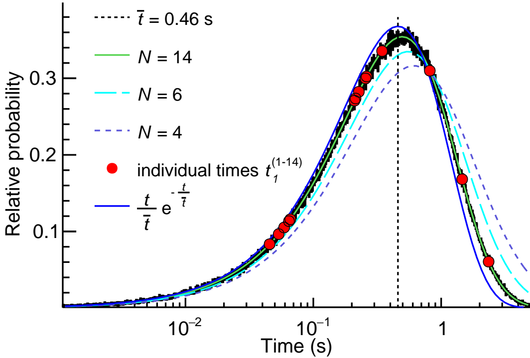
Figure A.5: (Color online) Relative probability for times t that originate from an exponential distribution with a decay constant that is estimated from a low-statistics measurement (black). The number of data points used for determination of the likelihood function of the decay constant \tau is N = N_1 = 14 and the corresponding average lifetime is \bar{t} = \bar{t}_1 = 0.459 s. The histogram is based on 10^5 simulated sets of chains. The analytic expression (Eq. A.1) for the corresponding probability density function (solid line, light green) is also shown. For reference, the probability density function for times from an exponential decay with a known decay constant is shown (solid line, dark blue). Probability density functions for cases where the lifetime was determined from N = 6 and N = 4 data points are also shown. The fourteen markers (circular, red) indicate the individual fourteen lifetimes t_1^{(1-14)} in decay step j = 1 of the fourteen short chains and their corresponding \text{FoM}_1^{(1-14)} .
