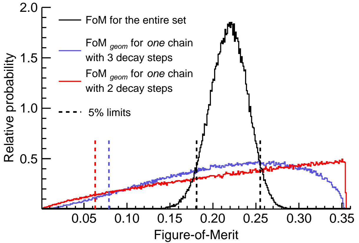
Figure A.6: (Color online) Relative probability of FoM values: FoM for an entire data set of fourteen chains with similar characteristics as the experimental fourteen short chains (black), \text{FoM}_{geom} for one of the recoil- \alpha - \alpha -SF chains (blue), and \text{FoM}_{geom} for one of the recoil- \alpha -SF chains (red). A selection of the respective 5% limits (dashed lines) are also shown. The histograms are based on 10^5 simulated sets of chains.
