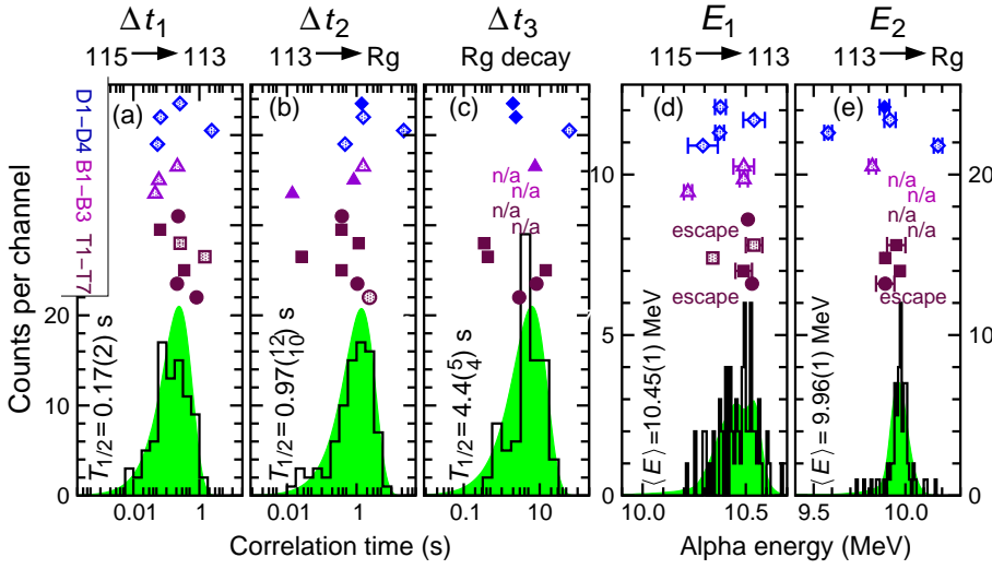
Figure 1: (Color online) Correlation times [(a)-(c)] and \alpha -energy spectra [(d) and (e)] of decay chains observed in the reaction ^{48}\text{Ca}+^{243}\text{Am} . The term “ \alpha energy” includes possible summation with energy deposited by conversion or Auger electrons. The black histograms are reference spectra and relate to experimental data from the 96 chains associated with the 3n evaporation channel ^{288}115 in Refs. [7, 8, 12]. The shaded areas in panels (a)-(c) are the corresponding time distributions. The shaded areas in panels (d) and (e) are the energy distributions derived from Monte Carlo simulations as outlined in Refs. [7, 32, 35]. The data points of the fourteen observed recoil- \alpha -( \alpha )-fission events are provided on top of each spectrum, labeled with an identifier according to Table 1. Filled symbols indicate measurement during beam-off periods. Diamonds refer to data from Ref. [12], triangles refer to data from Ref. [8], and squares and circles refer to the present data observed at 242.1 and 245.0 MeV mid-target beam energy, respectively. ‘n/a’ means ‘not applicable’, ‘escape’ denotes events with low-energy detection solely in the implantation DSSSD.
