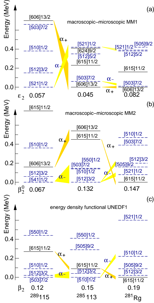
Figure 3: (Color online) Nuclear structure predictions of low-lying states in ^{289}\text{115} , ^{285}\text{113} , and ^{281}\text{Rg} . Panels (a) and (b) are based on two different macroscopic-microscopic approaches, MM1 [51, 52] and MM2 [53]. Panel (c) originates from the self-consistent Skyrme energy density functional UNEDF1 [55, 56]. The results from UNEDF1 SO are similar to MM2 [56]. Proton single-particle states are labeled with their asymptotic Nilsson quantum numbers [Nn_z\Lambda]\Omega . Full (black) lines represent positive-parity states, dashed (blue) lines negative-parity states. Selected \alpha -decay sequences among high- \Omega positive-parity ( \alpha_+ ) and low- \Omega negative-parity ( \alpha_- ) states are indicated by shaded areas. \epsilon_2 , \beta_2^0 , \beta_2 , respectively, denote predicted quadrupole deformations.
