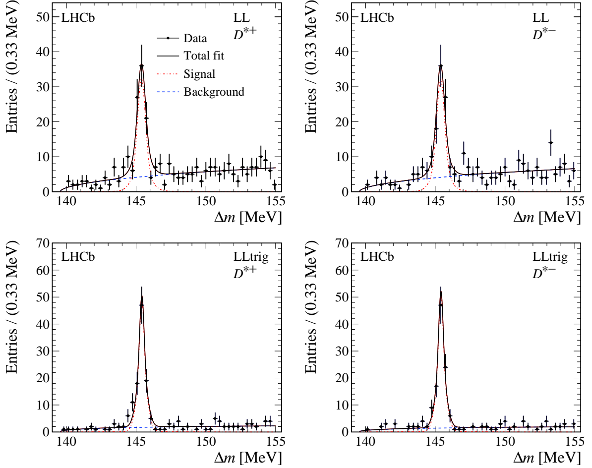
Figure 2: Distributions of \Delta m split into (left) D^{*+} , (right) D^{*-} and (top) LL, (bottom) LLtrig, including the fit function. The solid (black) line corresponds to the total fit, the dashed (blue) line corresponds to the background, and the dash-dotted (red) line represents the signal contribution.
