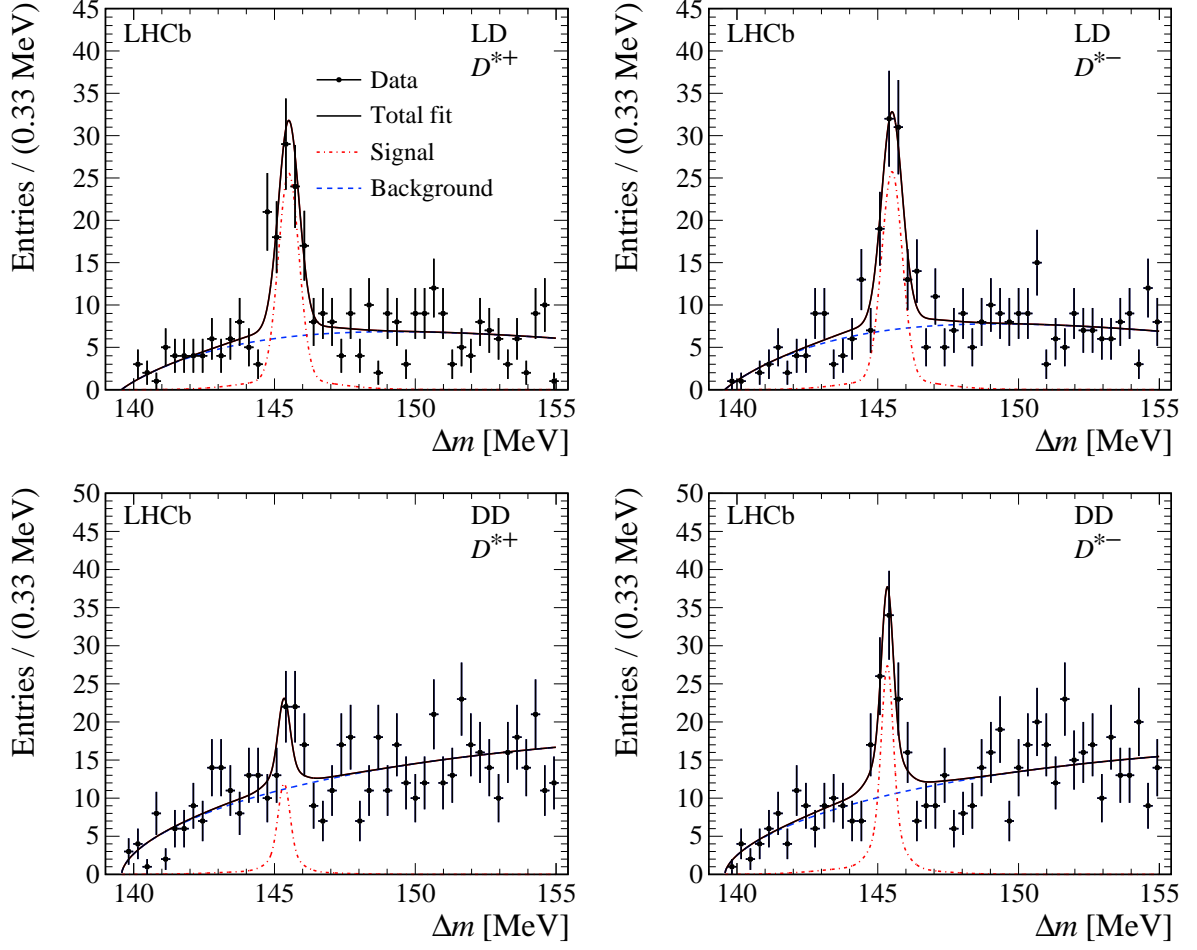
Figure 3: Distributions of \Delta m split into (left) D^{*+} , (right) D^{*-} and (top) LD, (bottom) DD, including the fit function. The solid (black) line corresponds to the total fit, the dashed (blue) line corresponds to the background, while the dash-dotted (red) line represents the signal contribution.
