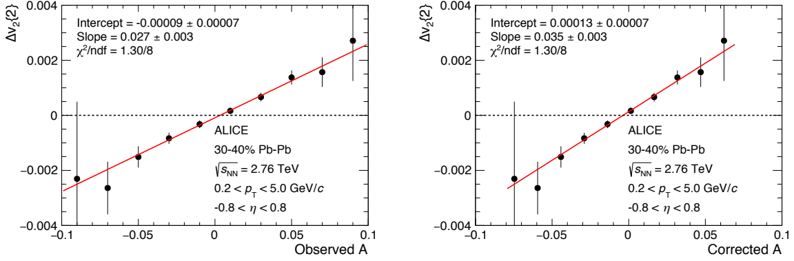
Fig. 2: (Color online) v_2 = v_2^- - v_2^+ as a function of the observed (left) and corrected (right) event charge asymmetry A in the 30–40% centrality class. Statistical uncertainties only.
