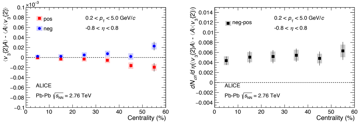
Fig. 5: (Color online) Three-particle correlator for the third harmonic (left panel) for positive (red squares) and negative (blue circles) particles, and the charge difference multiplied by dN_{\text{ch}}/d\eta (right panel). Statistical (systematic) uncertainties are indicated by vertical bars (shaded boxes).
