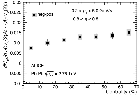
Fig. 4: Charge difference of the three-particle correlator for the second harmonic as a function of centrality, multiplied by dN_{ch}/d\eta [39]. Statistical (systematic) uncertainties are indicated by vertical bars (shaded boxes).
