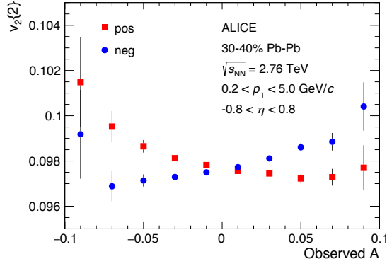
Fig. 1: (Color online) Harmonic coefficients v_2^+ (red squares) and v_2^- (blue circles) as a function of the observed event charge asymmetry A in the 30–40% centrality class. Statistical uncertainties only.
