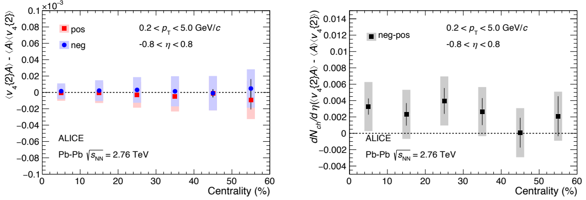
Fig. 6: (Color online) Three-particle correlator for the fourth harmonic (left panel) for positive (red squares) and negative (blue circles) particles, and the charge difference multiplied by dN_{\text{ch}}/d\eta (right panel). Statistical (systematic) uncertainties are indicated by vertical bars (shaded boxes).
