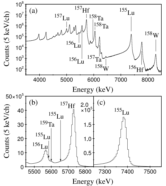
FIG. 1: (a) Energy spectrum of decays occurring within 700 ms of a recoil implantation in the same DSSD pixel. (b) The spectrum in (a) expanded around the \alpha -decay peaks of the (11/2^-) and (1/2^+) states in ^{155}\text{Lu} . (c) The spectrum in (a) expanded around the \alpha -decay peak of the (25/2^-) state.
