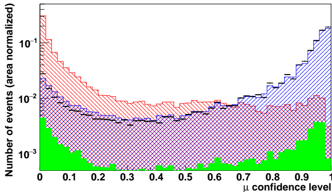
FIG. 2. Distribution of the \mu_{CL} variable for \nu_{\mu} CC (blue), \nu_e CC (red), and NC events (green) from the MC are overlaid with data (black). The data, \nu_{\mu} CC and \nu_{\mu} NC histograms are first normalized by protons on target. Then, these three histograms are scaled by one over the number of \nu_{\mu} CC events in order to preserve their relative proportions. The \nu_e CC histogram is area normalized to compare with the \nu_{\mu} CC histogram. The pink arrow represents the lower cut value on the \mu_{CL} that defines the \nu_{\mu} event selection.
