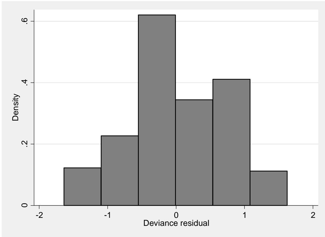
Figure S1: Histogram of the deviance residuals from the mixed effects model.
