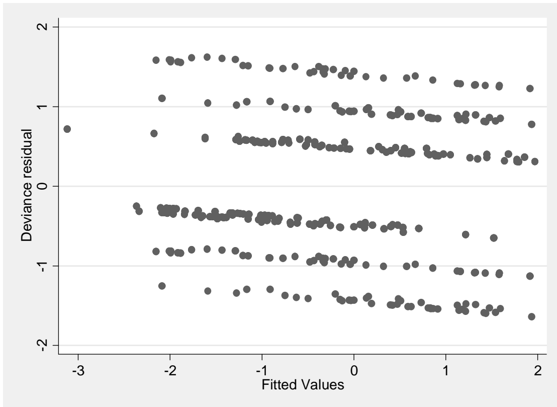
Figure S2: Scatter plot of the deviance residuals from the mixed effects model against the linear predictors of the fixed effects portion of the mixed effects model
