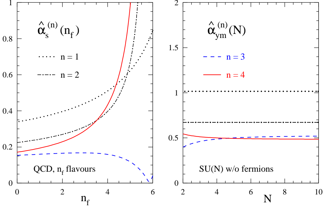
Figure 3: The values (3.13) and (3.14) of the coupling constants of QCD (left) and pure SU( N ) Yang-Mills theory (right) for which the absolute size of the N^n LO contribution to the beta function is a quarter of that of the N^{n-1} LO term for n = 1, 2, 3 (dashed curves) and 4 (solid curves).
