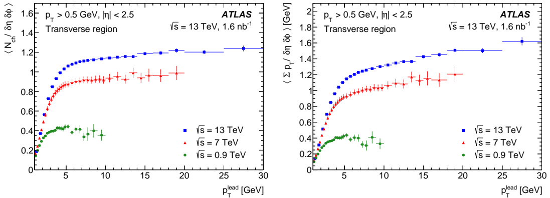
Figure 7: Mean charged-particle multiplicity (left) and \sum p_{\text{T}} (right) densities as a function of transverse momentum of the leading charged particle measured for \sqrt{s} = 0.9, 7 \text{ TeV} [1] and 13 TeV centre-of-mass energies. The fiducial acceptance definitions of the \sqrt{s} = 0.9 and 7 TeV measurements did not exclude charged strange baryons, but this effect is limited to a few percent at most.
