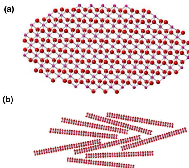
Fig. 2 Structural model. (a) Top view of the ordered region within a single \text{MnO}_2 layer, from which the powder diffraction pattern in Fig. 1 was calculated. Magenta – manganese; red – oxygen, (b) Schematic profile view of a possible arrangement of the ordered regions within layers of \text{Na}_{0.35}\text{MnO}_2 .
