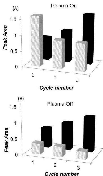
Figure 3: Changes in the peak area of the Au 0 (2095 cm -1 , grey) and Au 5+ (2120 cm -1 , black) species during (A) plasma on; (B) plasma off cycles.
