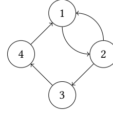
Figure 1: The lower bound example for n = 2 .
