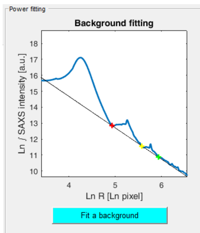
Figure 5: Power function background fitting. The azimuthally-integrated scatter signal (blue) is fitted with a power-law background function (black). User-selected fitting points are shown as red, yellow and green crosses.
