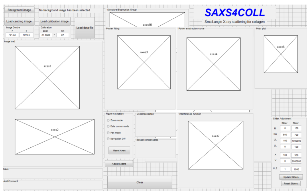
Figure 1: Layout of the SAXS4COLL GUI, illustrating the positions of the main processing and display windows, including: image display windows (axes 1 and 2), background fitting and display windows (axes 3 and 4), fibre orientation plot window (axes 6) and collagen fibril lattice function display window (axes 7).
