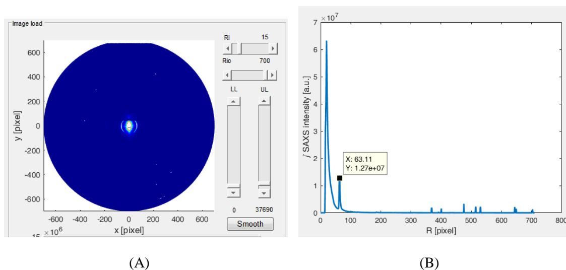
Figure 4: Interactive calibration using rat-tail tendon collagen. (A) Calibrant SAXS pattern and radial SAXS signal displayed in the SAXS4COLL GUI. (B) Manual selection of collagen meridional first order peak position to be used for calibration.
