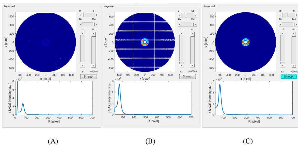
Figure 3: Removal of outliers and recovery of undetected areas of unprocessed patterns. (A) Original unprocessed image. (B) Adjusting slider limits, the lower limit (LL) threshold has been set to 6.1 such that undetected data (in this case from detector gaps) appears as white areas. (C) The same pattern after compensation. SAXS azimuth integrated signal is shown under each pattern.
