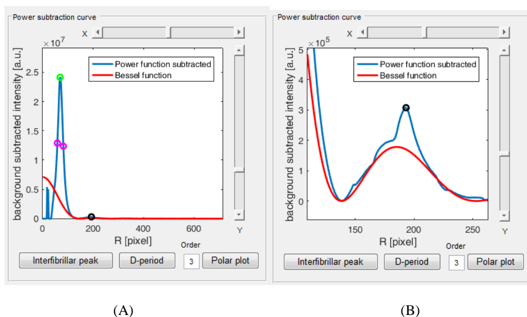
Figure 6: Collagen peak detection and fibril transform (Bessel function) fitting. (A) Power-function subtracted data with fitted Bessel function curve and the interfibrillar peak (green circle) and 3rd order meridional peak (black circle) detected. Magenta circles show the detected HHW limits. (B) Expanded view of the Bessel function fitting.
