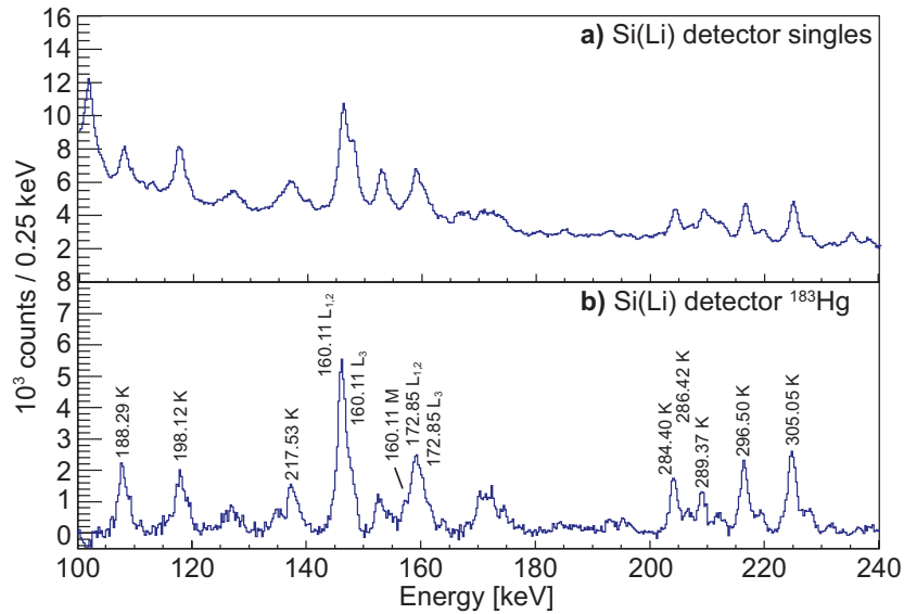
Figure 2. (Colour online) Spectrum of conversion electrons measured with the Si(Li) detector inside of the chamber of the HIGH-TATRA system: a) total singles spectrum and b) spectrum attributed to the decay of ^{183}\text{Hg} deconvoluted using time-stamped data, see the text for details.
