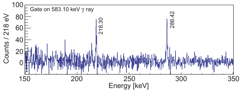
Figure 12. (Colour online) Spectrum of \gamma rays detected in prompt coincidence with the 583.10 keV \gamma rays.
