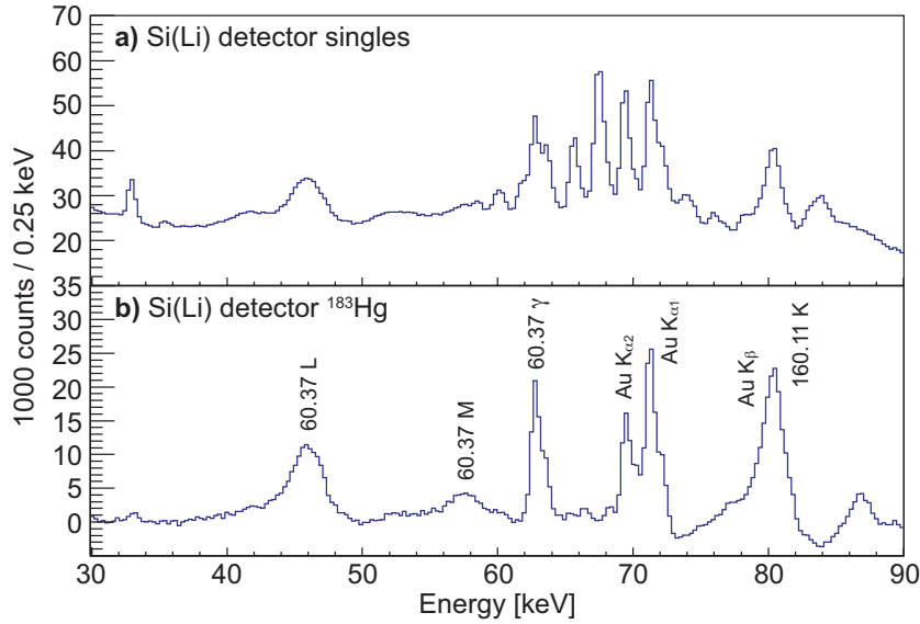
Figure 8. (Colour online) Spectrum of low-energy \gamma rays, characteristic x rays and conversion electrons measured with the Si(Li) detector inside of the chamber of the HIGH-TATRA system: a) total singles spectrum and b) spectrum attributed to the decay of ^{183}\text{Hg} deconvoluted using time-stamped data, see the text for details. Note that the energy calibration of the spectra shown is for conversion electrons. The calibration for \gamma rays and x rays differs due to the bias on the detector (-500 V), implantation depth into the metallic tape and to dead layer of the Si(Li) detector.
