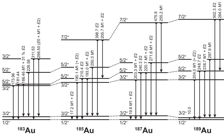
Figure 16. The systematics of the bands built on the low-lying, low-spin, positive-parity states of 2d_{3/2} and 3s_{1/2} configurations in odd-Au isotopes. Data are taken from this work and from [8, 11].
