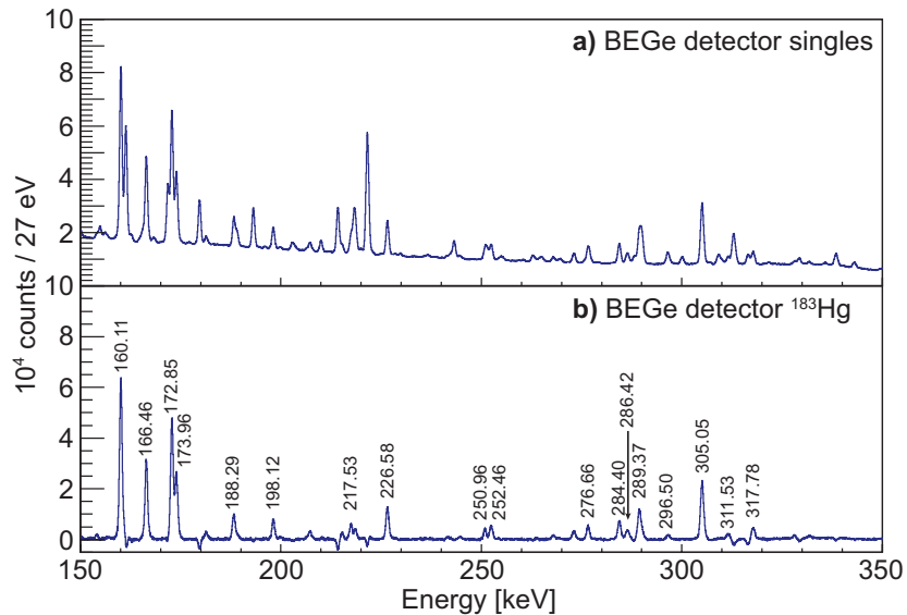
Figure 3. (Colour online) Spectrum of \gamma rays measured with the BEGe detector: a) total singles spectrum and b) spectrum attributed to the decay of ^{183}\text{Hg} deconvoluted using time-stamped data, see the text for details.
