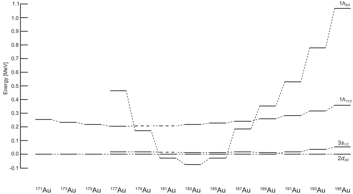
Figure 1. Systematics of 3s_{1/2} , 2d_{3/2} , 1h_{11/2} and 1h_{9/2} proton configurations in neutron-deficient odd-Au isotopes. The data are taken from [5, 8, 11, 13, 16, 26, 27, 28].
