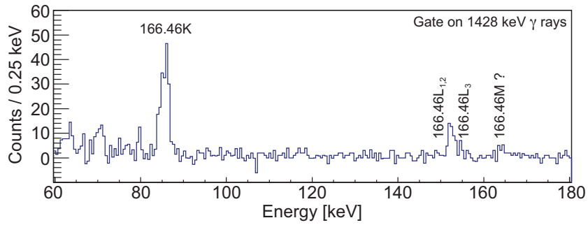
Figure 10. (Colour online) Spectrum of conversion electrons detected in prompt coincidence with the 1428 keV \gamma rays.
