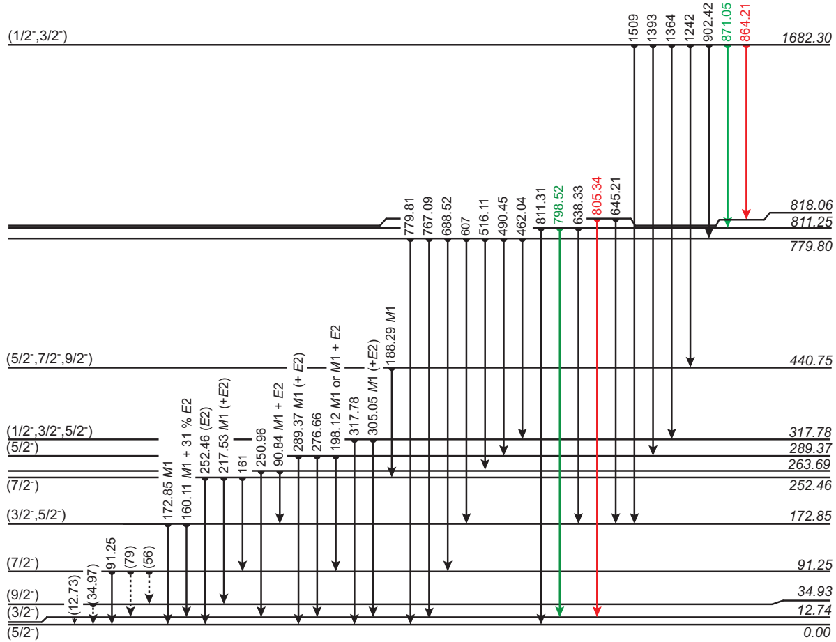
Figure 5. (Colour online) Partial level scheme of low-lying, negative-parity states associated with the 1h_{9/2} and 2f_{7/2} intruder configurations in the ^{183}\text{Au} isotope deduced from the present work. The \gamma -ray energies of transitions are given. See Table 2 for intensities and multiplicities of transitions. Transition energies were determined using the \gamma -singles spectrum detected with the BEGe detector. Transitions with energies given as integer numbers are either weak, dominated by other \gamma lines, or their energy exceeds 980 keV, which was the upper limit for the BEGe detector in this experiment, see the text for details. Their location in the scheme is proven by the \gamma - \gamma coincidences. All states are populated via the decay of the 1682.30 keV state, see the text for details. Decay paths used for the localisation of the critical 60.73 keV transition connecting intruder and proton-hole states are highlighted with red and green colour, see the text for details.
