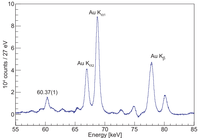
Figure 7. (Colour online) Spectrum of low-energy \gamma rays detected with the BEGe detector that are unambiguously attributed to ^{183}\text{Hg} decay by deconvolution of time-stamped data, see the text and Ref. [32] for details.
