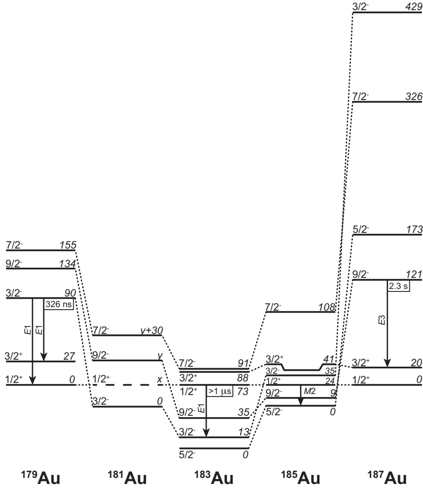
Figure 14. Systematics of 9/2^- , 7/2^- , 3/2^- , and 1/2^- states associated with the 1h_{9/2} and 2f_{7/2} intruder configurations and 1/2^+ , and 3/2^+ states of 2d_{3/2} and 3s_{1/2} proton-hole configurations in odd-Au isotopes. Important parity-changing transitions that are connecting above intruder and proton-hole configurations are indicated. Note that the half life of the 1/2^+ , 24 keV state in ^{185}\text{Au} is unknown and only inadequate data [50] are available for the ^{181}\text{Au} isotope. The data are taken from this work and from [8, 11, 28, 51]
