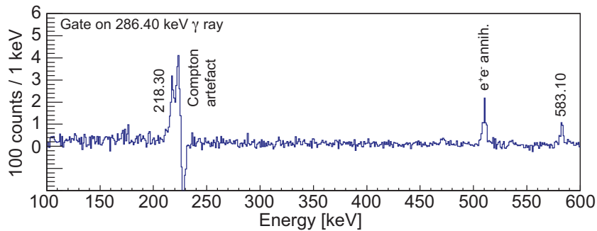
Figure 13. (Colour online) Spectrum of \gamma rays detected in prompt coincidence with the 286.40 keV \gamma rays. The structure denoted as “Compton artefact” is due to scattering of 511 keV electron-positron annihilation quanta between two germanium detectors.
