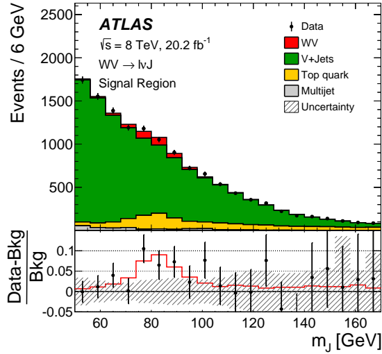
Figure 5: The observed m_J distribution in the WV \rightarrow \ell\nu J signal region, overlaid with the post-fit background and signal estimates. The hatched band indicates the total uncertainty of the fit result.
