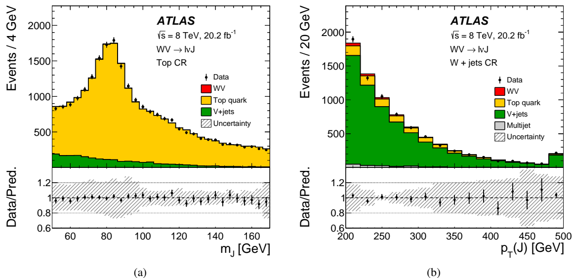
Figure 3: Comparison between data and prediction in the WV \rightarrow \ell\nu J channel for (a) m_J in the top CR, and (b) p_T(J) in the W + \text{jets} CR. A scale factor is applied to the top-quark background prediction in the top CR and the W + \text{jets} CR, and a scale factor is applied to the W + \text{jets} background prediction (which is part of the “ V + \text{jets} ” histogram) in the W + \text{jets} CR. The hatched bands indicate the systematic uncertainty of the prediction. For the V + \text{jets} component, only shape systematic uncertainties are included in the bands.
