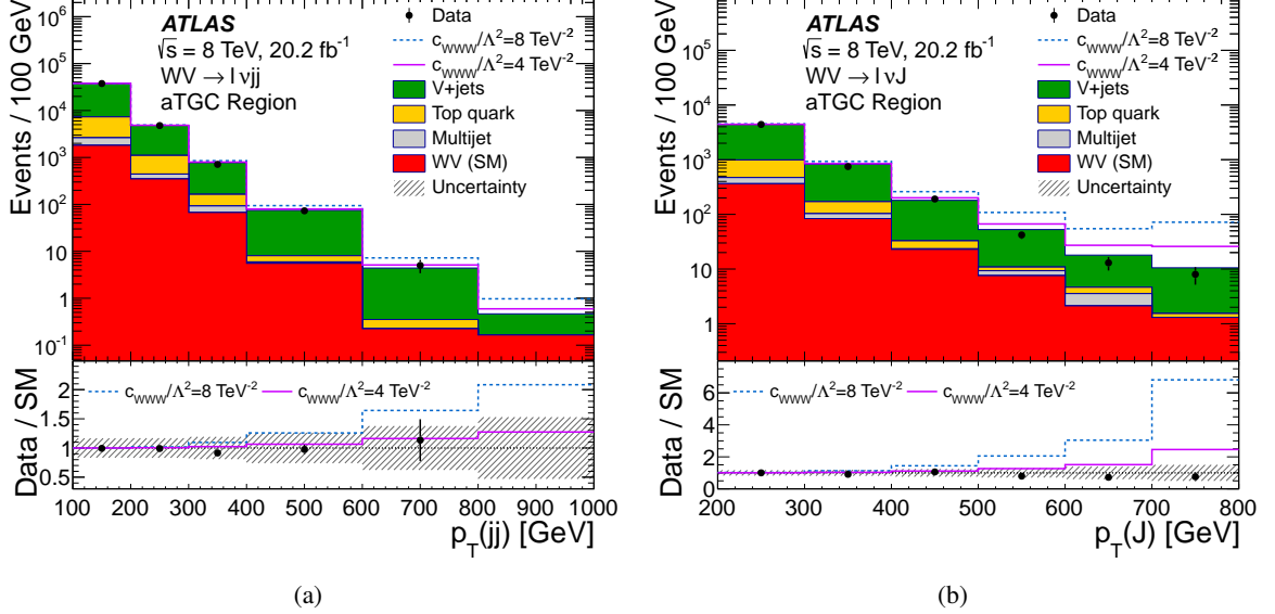
Figure 7: The observed (a) p_T(jj) distribution in the WV \rightarrow \ell\nu jj aTGC signal region, and (b) p_T(J) distribution in the WV \rightarrow \ell\nu J aTGC signal region, overlaid with the background and signal prediction. The expected BSM enhancements due to anomalous values of the EFT parameter c_{WWW}/\Lambda^2 are also shown, for c_{WWW}/\Lambda^2 = 4 \text{ TeV}^{-2} and c_{WWW}/\Lambda^2 = 8 \text{ TeV}^{-2} . The hatched bands indicate the systematic uncertainty in the SM prediction. The histograms are displayed with the binning that is used for the computation of the confidence intervals for the aTGC and EFT parameters. The last bin includes overflow.
