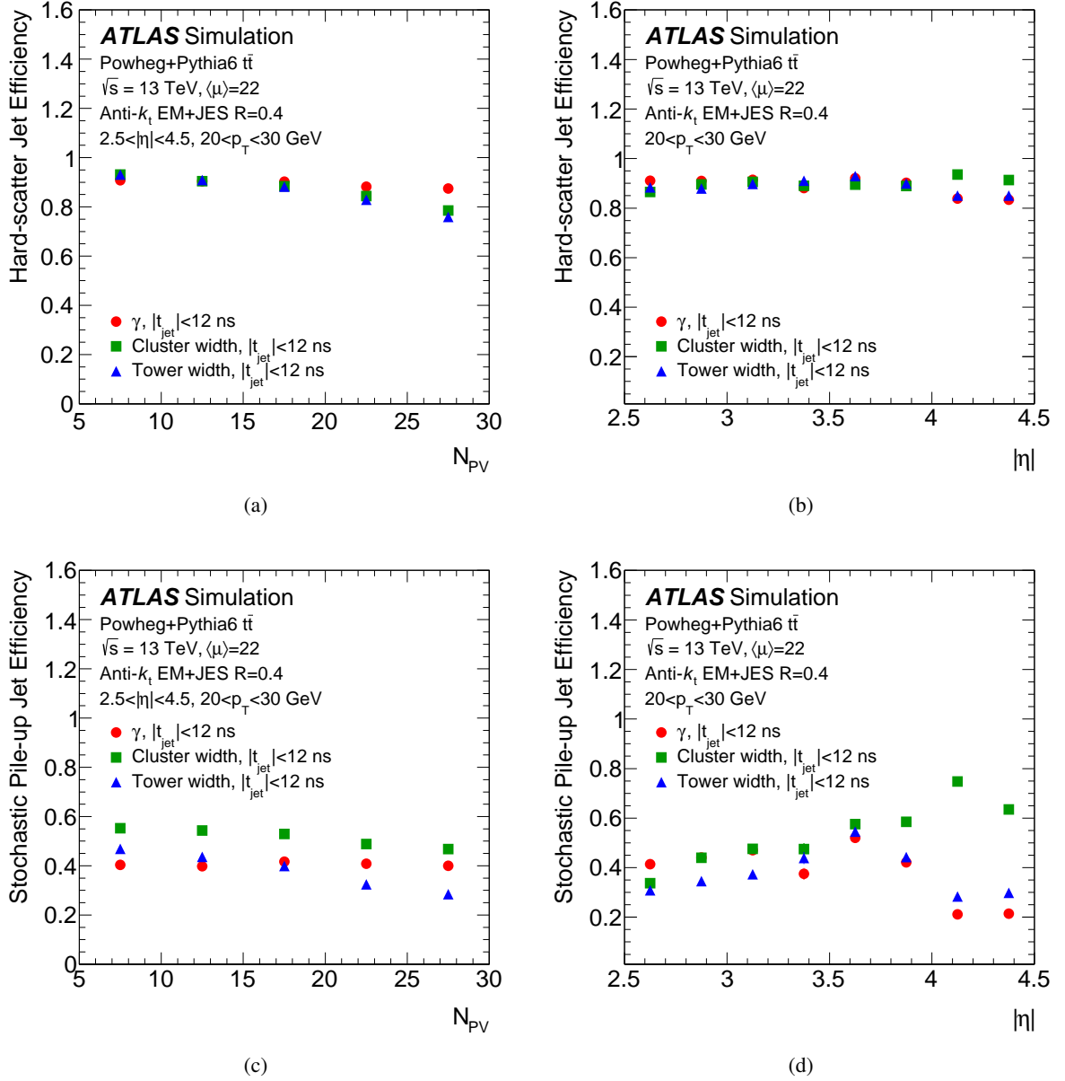
Figure 10: Hard-scatter jet efficiency as a function of (a) number of reconstructed primary vertices N_{PV} and (b) pseudorapidity |\eta| , as well as stochastic pile-up jet efficiency as a function of (c) number of reconstructed primary vertices N_{PV} and (d) pseudorapidity |\eta| at 90% efficiency of selecting hard-scatter jets in simulated t\bar{t} events.
