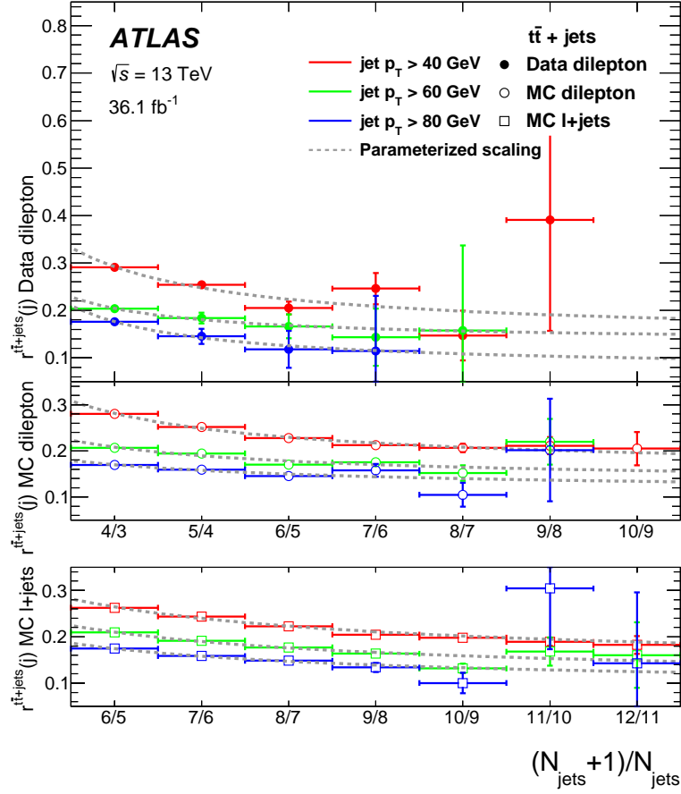
Figure 5: The ratio of the number of events with (j + 1) jets to the number with j jets in dileptonic and semileptonic t\bar{t}+jets events, used to validate the jet-scaling parameterization. Each panel shows the ratio for data or MC simulation with the fitted parameterization overlaid as a line. In the case of pure “staircase scaling”, the shown ratio would be a constant. The uncertainties shown are statistical.
