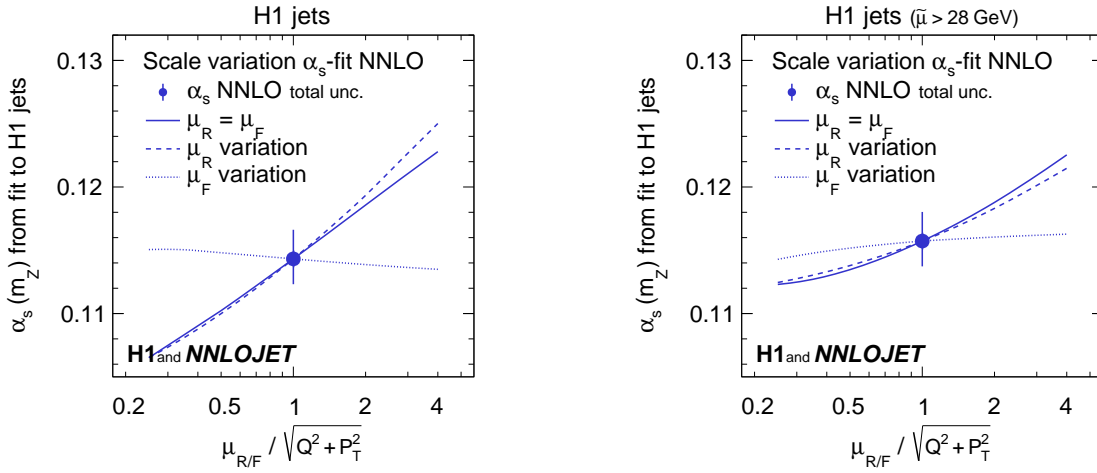
Figure 7: Dependencies of the fitted values of \alpha_s(m_Z) as a function of the scale factors for the H1 jets fit (left) and the H1 jets fit with \tilde{\mu} > 28 \text{ GeV} (right). Further details are given in the caption of figure 6.
