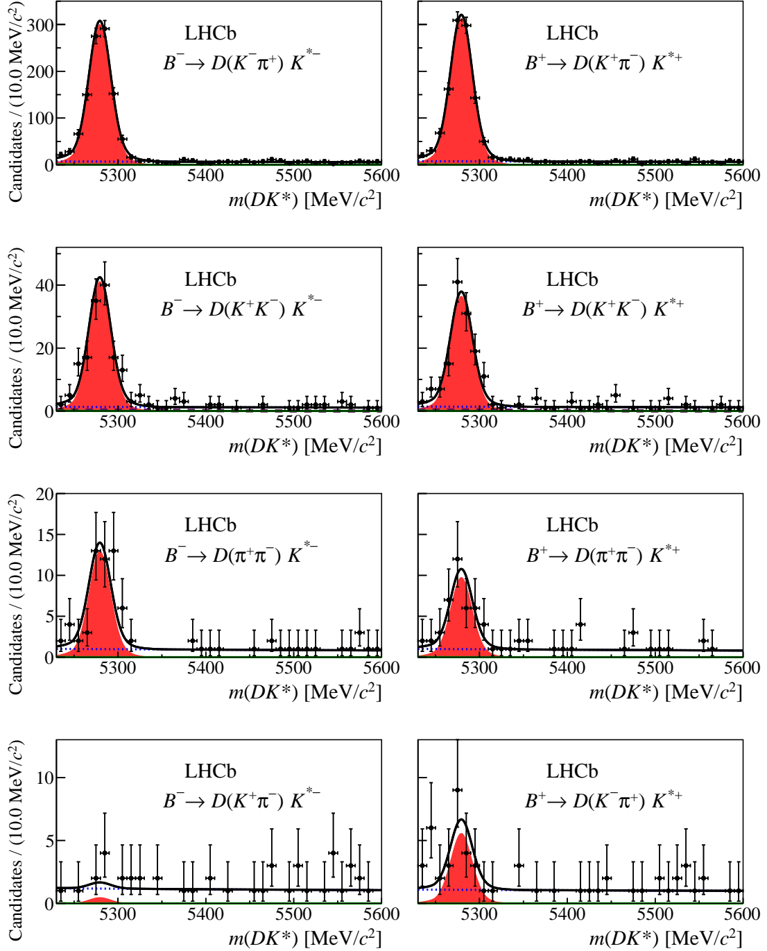
Figure 2: Result of fits to data for the two-body decay modes with Run 1, Run 2, long and downstream categories summed for presentation. The signal is represented by the red shaded area, the combinatorial background by the dotted blue line and the partially reconstructed background by the solid green line. In the D^0 \rightarrow K^+ K^- fits the \Lambda_b^0 \rightarrow \Lambda_c^+ K^{*-} background is represented by the dashed purple line. The total fit is given by the black line.
