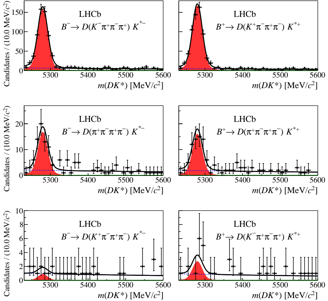
Figure 3: Result of fits to data for the four-body decay modes with Run 1, Run 2, long and downstream categories summed for presentation. The signal is represented by the red shaded area, the combinatorial background by the dotted blue line and the partially reconstructed background by the solid green line. The total fit is given by the black line.
