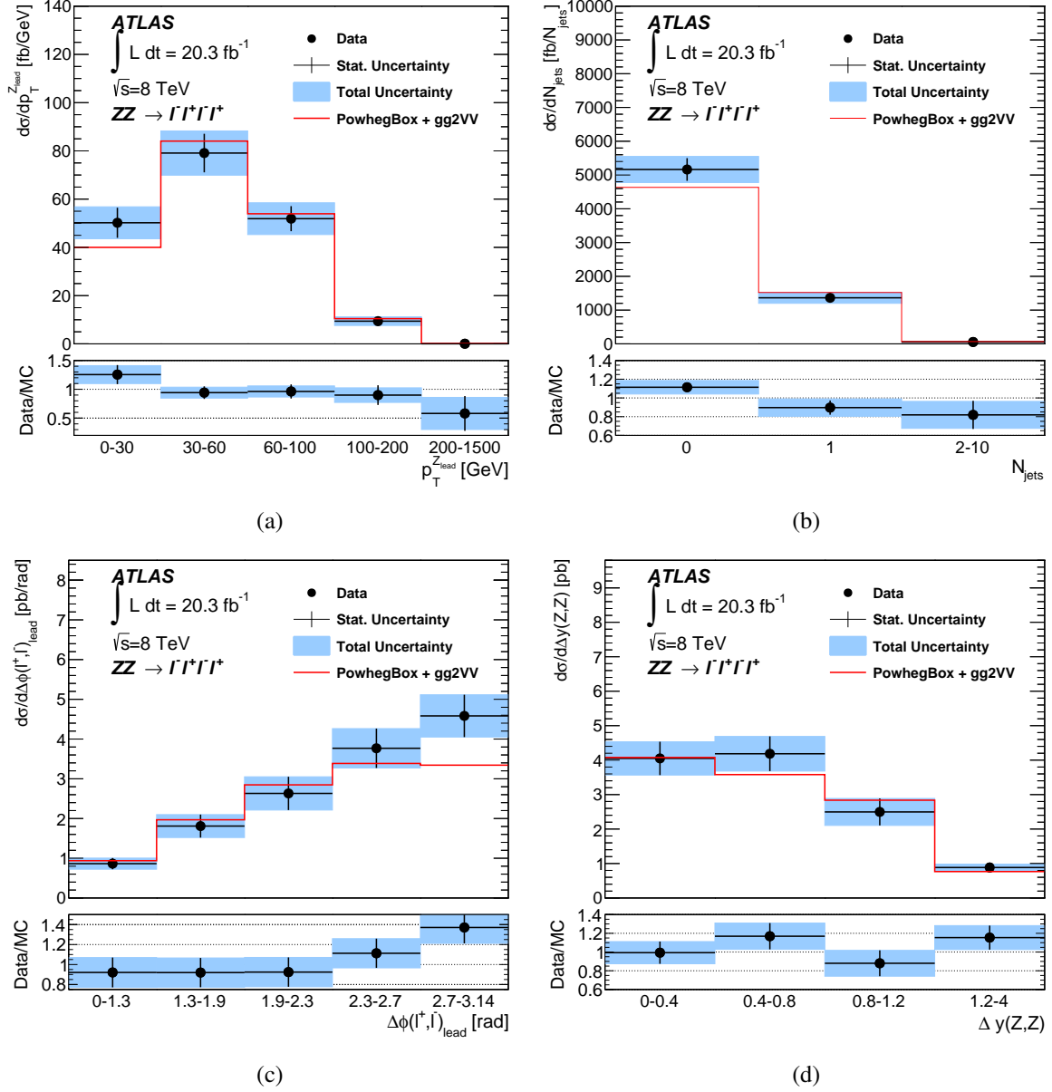
Figure 6: The measured differential cross-section distributions (black points) normalized to the bin width for (a) p_T^Z , (b) N_{\text{jets}} , (c) \Delta\phi(\ell^+, \ell^-)_{\text{lead}} and (d) \Delta y(Z, Z) in the ZZ \rightarrow \ell^- \ell^+ \ell^- \ell^+ channel, unfolded within the total phase space, compared to the theory predictions of PowhegBox and gg2VV (red line). The vertical error bars show the respective statistical uncertainties, while the light blue error bands express the statistical and systematic uncertainties of the measurements added in quadrature.
