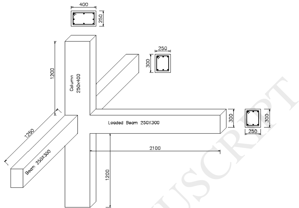
Fig. 5 Typical concrete dimensions
