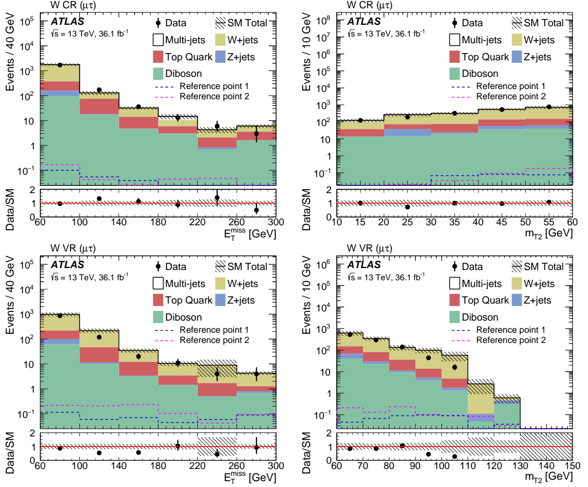
Figure 4: The E_T^{\text{miss}} (left) and m_{T_2} (right) distributions in the W -CR (top) and W -VR (bottom) regions. The SM backgrounds other than multi-jet production are estimated from MC simulation. The contribution of W +jets events is scaled to the fit result. The multi-jet contribution is estimated from data using the OS - SS method. The hatched bands represent the combined statistical and systematic uncertainties of the total SM background. For illustration, the distributions of the SUSY reference points defined in Section 3 are also shown as dashed lines. The lower panels show the ratio of data to the SM background estimate. The last bin includes the overflow events.
