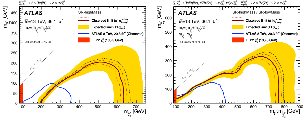
Figure 7: The 95% CL exclusion contours for simplified models with \tilde{\chi}_1^+\tilde{\chi}_1^- production (left) and production of \tilde{\chi}_1^+\tilde{\chi}_1^- and \tilde{\chi}_1^+\tilde{\chi}_2^0 (right). The text provides details of exclusion curves and uncertainty bands. The LEP limit on the chargino mass is also shown. Results are compared with the observed limits obtained by previous ATLAS searches [29] as blue contours.
