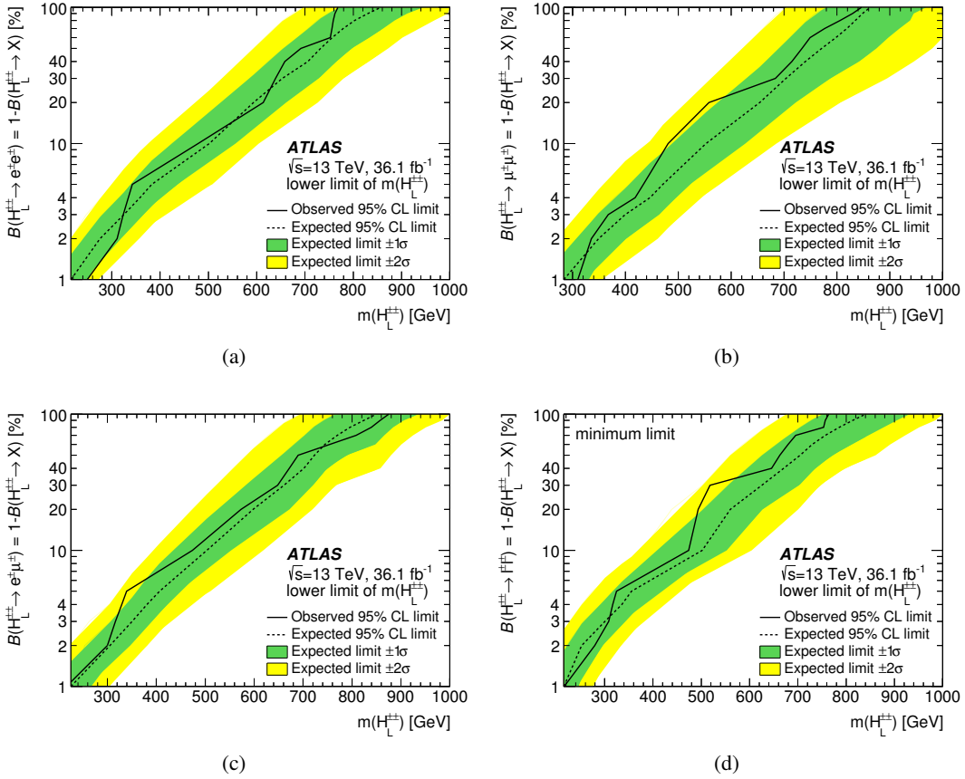
Figure 13: Lower limit on the H_L^{\pm\pm} boson mass as a function of the branching ratio B(H_L^{\pm\pm} \rightarrow \ell^\pm \ell^\pm) . Several cases are presented: (a) H_L^{\pm\pm} decays only into electrons and "X", (b) H_L^{\pm\pm} decays only into muons and "X", and (c) H_L^{\pm\pm} decays only into electron–muon pairs and "X", with "X" not entering any of the signal regions. Plot (d) shows the minimum observed and expected limit as a function of B(H_L^{\pm\pm} \rightarrow \ell^\pm \ell^\pm) .
