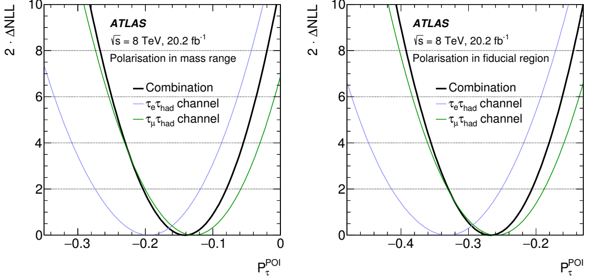
Figure 6: Likelihood profiles of P_\tau^{\text{POI}} for the fits that extract the polarisation in the mass-selected region of 66 < m_{Z/\gamma^*} < 116 GeV (left) and in the fiducial region (right). The profiles are shown separately for the fits in the \tau_e\text{-}\tau_{\text{had}} and \tau_\mu\text{-}\tau_{\text{had}} channels and for the combination.
