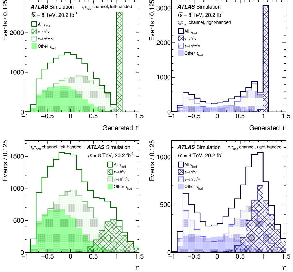
Figure 1: Charged asymmetry distributions as defined in Eq. (3) for left-handed (left) and right-handed (right) single-prong reconstructed \tau_{\text{had}} leptons in simulated Z/\gamma^* \rightarrow \tau\tau decays after the full event selection in the \tau_{\mu}\text{-}\tau_{\text{had}} channel. The charged asymmetry is calculated from stable-particle-level (top) and reconstructed-detector-level (bottom) quantities. In addition to the inclusive distributions, the constituent distributions corresponding to generated \tau leptons that decay in the \tau \rightarrow h^{\pm}\nu and \tau \rightarrow h^{\pm}\pi^0\nu ( h^{\pm} denotes \pi^{\pm} or K^{\pm} ) modes are overlaid, as well as that of the remaining decay modes. The latter mainly consist of \tau \rightarrow h^{\pm}N\pi^0\nu decays, where N \geq 2 . The analysis does not, however, distinguish between the decay modes. The distributions are normalised according to their respective cross-sections. Here, the polarisation is taken from the simulation.
