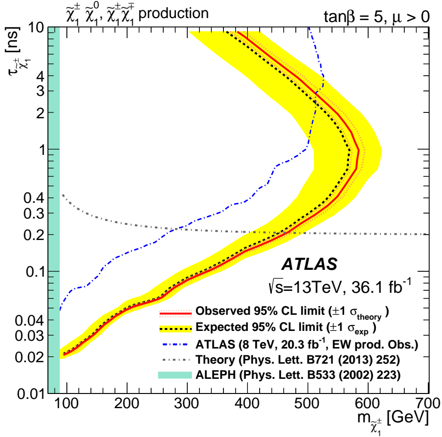
Figure 8: Exclusion limit at 95% CL obtained in the electroweak production channel in terms of the chargino lifetime ( \tau_{\tilde{\chi}_{\pm}^{\pm}} ) and mass ( m_{\tilde{\chi}_{\pm}^{\pm}} ). The yellow band shows the 1\sigma region of the distribution of the expected limits. The median of the expected limits is shown by a dashed line. The red line shows the observed limit and the orange dotted lines around it show the impact on the observed limit of the variation of the nominal signal cross-section by \pm 1\sigma of its theoretical uncertainties. Results are compared with the observed limits obtained by the previous ATLAS search with disappearing tracks and tracklets [19] and an example of the limit obtained at LEP2 by the ALEPH experiment [61]. The chargino lifetime as a function of the chargino mass is shown in the almost pure wino LSP scenario at the two-loop level [62].
