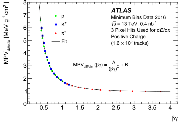
Figure 2: MPV_{dE/dx} as a function of \beta\gamma obtained with a sample of minimum-bias data from 2016, for positively charged tracks with three pixel hits used to calculate the dE/dx . This data sample amounts to about 0.4 \text{ nb}^{-1} . For each kaon and proton, the \beta\gamma value is corrected for the effect of multiple scattering. A fit to the MPV_{dE/dx} dependence on \beta\gamma with an empirical three-parameter function MPV_{dE/dx} = A/(\beta\gamma)^C + B motivated by Bethe–Bloch relation is also shown. The values of the A, B and C parameters for tracks with different charge and different number of pixel hits are all compatible.
