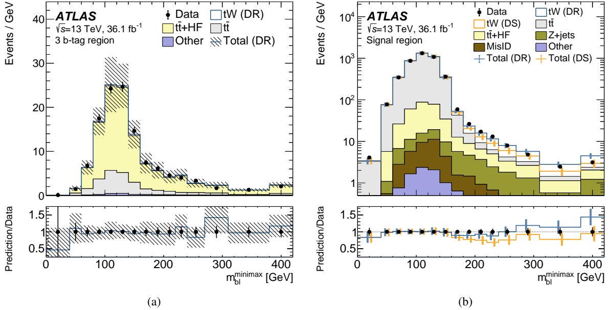
Figure 1: (a) The m_{b\ell}^{\text{minimax}} distribution in the three- b -tag region, constructed from the two b -jets with largest p_T . The predicted t\bar{t} +HF contribution from simulation is scaled to match observed data in this region. The hashed band indicates the uncertainty on the total number of predicted events, where the DR scheme is used to estimate the minor contribution from the tW process. (b) The detector-level m_{b\ell}^{\text{minimax}} distribution, with signal selection and background estimation as described in the text. The total predicted events are shown for both the DR and DS definitions of the tW process, with uncertainties on the respective estimates indicated by separate error bars. Uncertainties include all statistical and systematic sources. The rightmost bin of each distribution includes contributions from events beyond the displayed axis limit.
