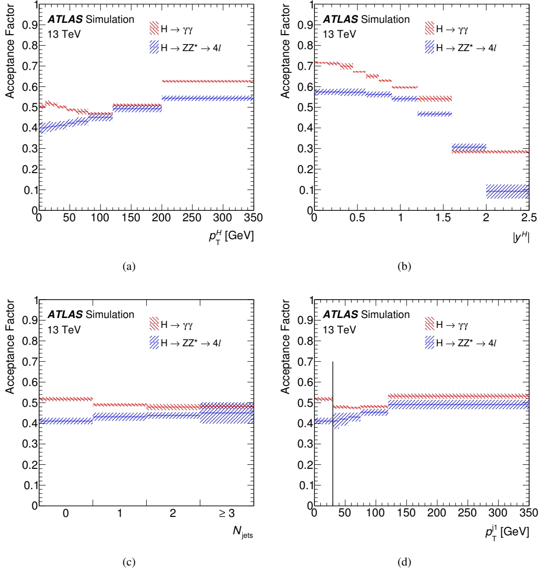
Figure 1: Acceptance factors for the extrapolation from the fiducial to the total phase space for the H \rightarrow \gamma\gamma decay channel (red) and the H \rightarrow ZZ^* \rightarrow 4l decay channel (blue), for (a) Higgs boson transverse momentum p_T^H , (b) Higgs boson rapidity |y^H| , (c) number of jets N_{\text{jets}} with p_T > 30 GeV, and (d) transverse momentum of the leading jet p_T^{j1} , including systematic uncertainties. The first bin in the p_T^{j1} distribution corresponds to the 0-jet bin in the N_{\text{jets}} distribution, as indicated by the black vertical line.
