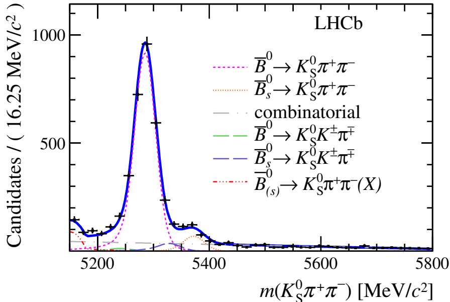
Figure 1: Invariant mass distributions of K_S^0\pi^+\pi^- candidates, summing the two years of data taking and the two K_S^0 reconstruction categories. The sum of the partially reconstructed contributions from B to open charm decays, charmless hadronic decays, \bar{B}^0 \rightarrow \eta' K_S^0 and charmless radiative decays are denoted \bar{B}_{(s)}^0 \rightarrow K_S^0\pi^+\pi^-(X) .
