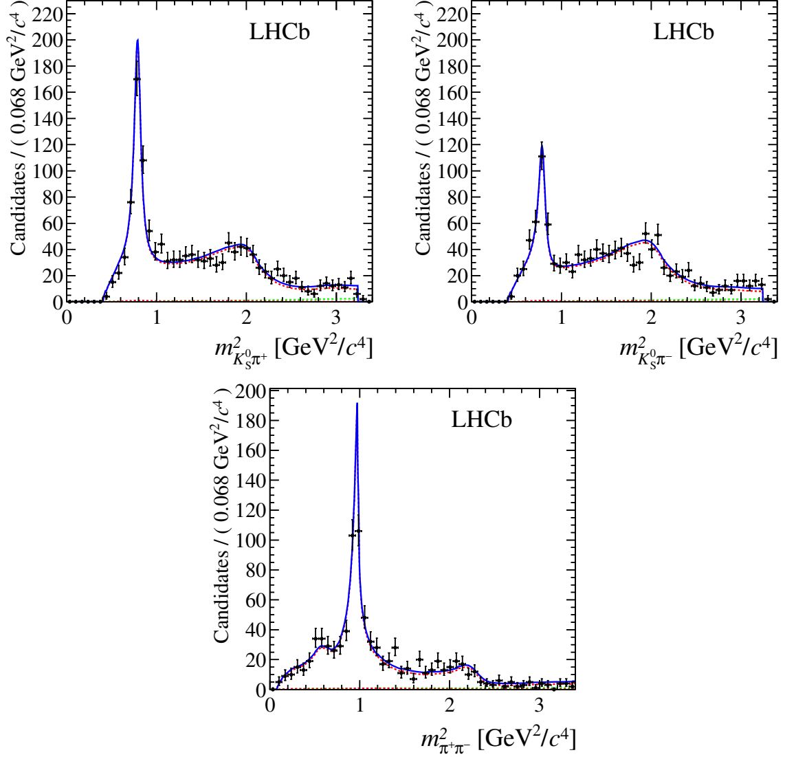
Figure 2: Projections of the sum of all data categories (black points) and the nominal fit function onto the DP variables (left) m_{K_S^0 \pi^+}^2 , (right) m_{K_S^0 \pi^-}^2 and (bottom) m_{\pi^+ \pi^-}^2 , restricted to the two-body low invariant-mass regions. The full fit is shown by the solid blue line and the signal model by the dashed red line. The observed difference is due to the (green) combinatorial and (light red) cross-feed background contributions, barely visible in these projections.
