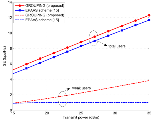
Fig. 3. SE performance versus transmit power
