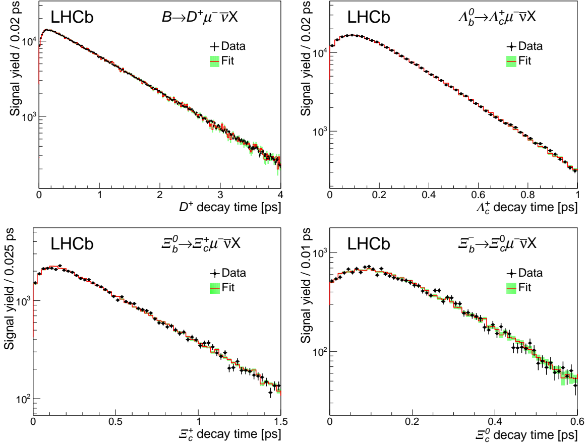
Figure 2: Decay-time spectra for (top left) D^+ signal in B \rightarrow D^+ \mu^- \bar{\nu}_\mu X , (top right) \Lambda_c^+ signal in \Lambda_b^0 \rightarrow \Lambda_c^+ \mu^- \bar{\nu}_\mu X , (bottom left) \Xi_c^+ signal in \Xi_b^0 \rightarrow \Xi_c^+ \mu^- \bar{\nu}_\mu X , and (bottom right) \Xi_c^0 signal in \Xi_b^- \rightarrow \Xi_c^0 \mu^- \bar{\nu}_\mu X candidate decays. Overlaid are the fit results, as described in the text, along with the uncertainties due to finite sizes of the simulated samples.
