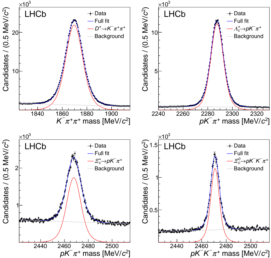
Figure 1: Invariant-mass distributions for candidate (top left) D^+ in B \rightarrow D^+ \mu^- \bar{\nu}_\mu X , (top right) \Lambda_c^+ in \Lambda_b^0 \rightarrow \Lambda_c^+ \mu^- \bar{\nu}_\mu X , (bottom left) \Xi_c^+ in \Xi_b^0 \rightarrow \Xi_c^+ \mu^- \bar{\nu}_\mu X , and (bottom right) \Xi_c^0 in \Xi_b^- \rightarrow \Xi_c^0 \mu^- \bar{\nu}_\mu X candidate decays. The results of the fits, as described in the text, are overlaid.
